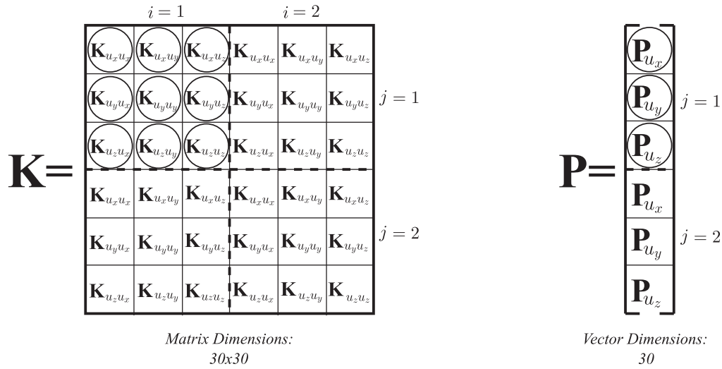
FIGURE 10 | Assembly of the general stiffness matrix and the general load vector.
