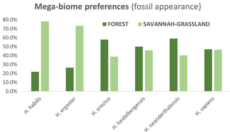
Figure 3.1 Mega-biome preferences in terms of time of fossil appearance. Forest: tropical forest, warm-temperate forest, temperate forest, boreal forest. Savannah-grassland: savannah and dry woodland, grassland and dry scrubland, dry tundra, tundra, barren.
