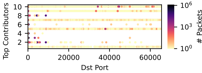
Fig. 9. TCP destination ports of internal erroneous traffic generated by the top-10 contributors.
