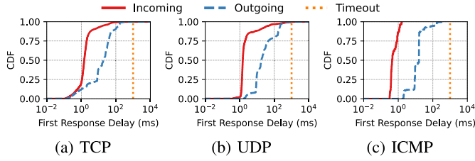
Fig. 11. First response delay of incoming and outgoing flows, measured in our campus network.
