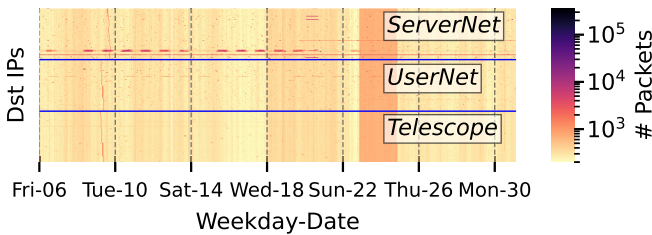
Fig. 8. Incoming traffic collected by CHAMALEONET and pure telescope (1-hour interval). Blue lines mark the three /24 subnets.
