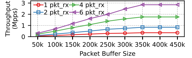
Fig. 13. Throughput of the FSD-NF under DoS workload.
