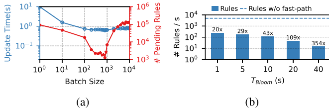
Fig. 14. (a) Batching amortizes gRPC call overhead, until the switch's processing time for rule installation becomes dominant. (b) The fast-path cuts the update rate on the slow-path by orders of magnitude, mitigating bottleneck #1.
