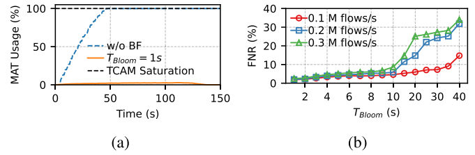
Fig. 15. (a) The Bloom filter (BF) bounds TCAM occupancy, whereas the baseline saturates the capacity shortly. (b) Empirical false negative rate of CHAMALEONET's filtering across different T_{\text{Bloom}} under adversarial traffic.
