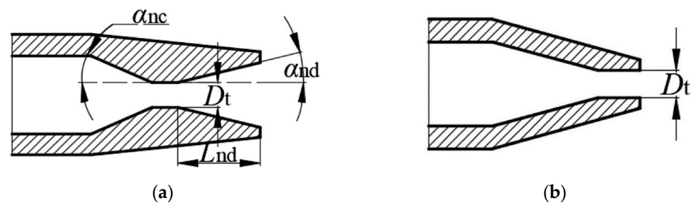
Figure 4. (a) Supersonic nozzle and (b) subsonic nozzle [39].
