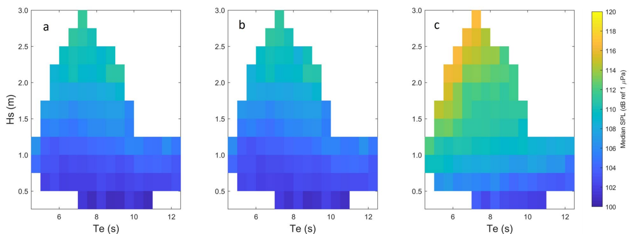
Fig. 1. Median sound pressure levels (10 Hz–96 kHz) as a function of significant wave height H_s and wave energy period T_e at: (a) Station 1 (110 m range), (b) Station 2 (170 m range), and (c) Station 3 (10 m range). Wave heights and periods are binned into 0.25 m and 0.5 s windows, respectively.
