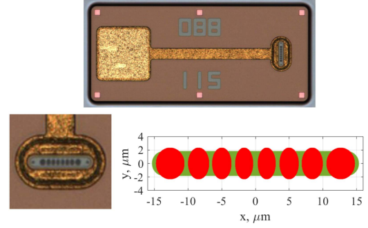
Fig. 6. Top view of the whole VCSEL chip. Bottom left: magnification on the rectangular VCSEL, with GRs and no dielectrics. The metal p-contact is formed by the two horizontal stripes above and below the GR array. Bottom right: a magnified schematic of the GR array (in red) and rectangular oxide aperture (in green). The dimensions of the rectangle are 30.5 \times 3.5 \mu\text{m}^2 .
