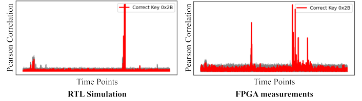
Fig. 3: CPA results for Ibex core running software AES. Left: RTL-derived structure-aware proxy. Right: FPGA measurements.
