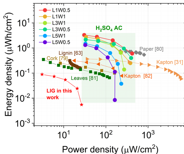
Fig. 6 Ragone plot comparing the performance of the devices of this paper with bio-derived 63,79–81 and Kapton-based 31,82 LIG supercapacitors from the literature.
