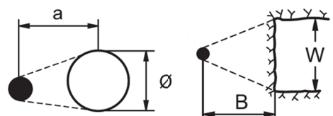
Fig. 2. Parameters for the design of the first quadrant of the cut. Adapted from [20]
