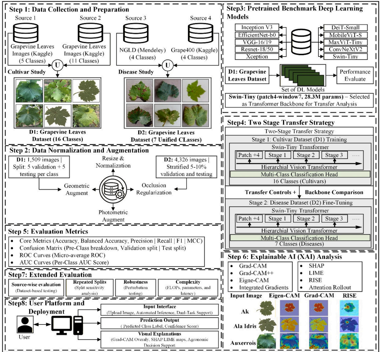
Fig. 1. End-to-end pipeline of the proposed unified deep learning framework, starting from cultivar and disease dataset construction, followed by preprocessing and augmentation, pretrained backbone benchmarking, Swin-Tiny selection as the transformer backbone for two-stage transfer analysis, transfer validation controls, backbone comparison, extended evaluation, post-hoc XAI analysis, and deployment through a lightweight image-to-decision platform.
