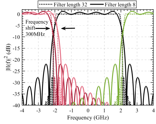
Fig. 3: Transmitter pulse frequency responses for the SC under test and its neighboring SCs in the frequency-resolved model, for a roll-off factor of 0.05 and two filter lengths, with and without a 300 MHz frequency offset in the left SC. The legend applies to all SCs.
