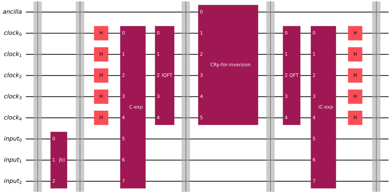
FIGURE 1. Circuit ideally implementing HHL algorithm ( n = 3 input qubits, n_c = 5 clock qubits and 1 ancilla qubit) for solving the problem discussed in the previous sections. “C-exp” stands for controlled exponentiation (or controlled Hamiltonian evolution), while “iC-exp” stands for its logical inverse. “CRy-for-inversion” stands for controlled rotation for eigenvalue inversion. Since this circuit does not include any measurements, it is suitable only for ideal (statevector) simulations.
