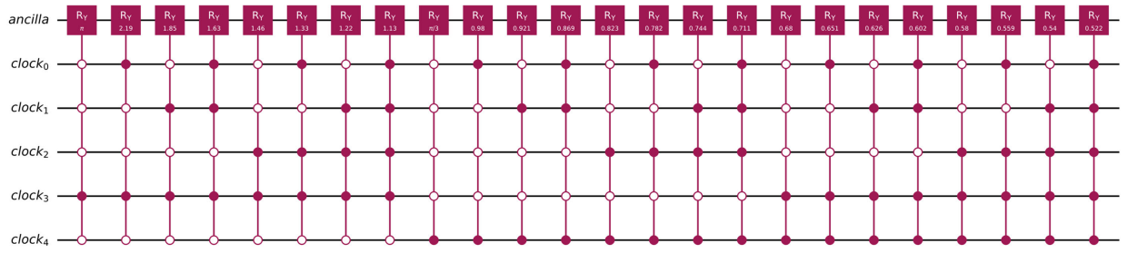
FIGURE 3. Circuit implementing controlled rotation on the ancilla qubit in the HHL algorithm with n_c = 5 clock qubits. As it is clear from the circuit, k_{(10)}^{\min} = 8 , which corresponds to k^{\min} = 1000 and is the controller condition of the first rotation block on the left. This circuit shows what is inside the block called “CRy-for-inversion” in Fig. 1.
