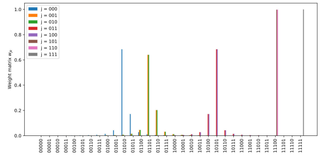
FIGURE 4. Normalized weights w_{jk} , where \sum_k w_{jk} = 1 for every j -th component of the spectral decomposition. It is worth noting that the binarization process implies (N_c - 1)\lambda_j^\Gamma \approx (k_j^\Gamma)_{(10)} , which introduces some spread in the spectral distribution of the binarized eigenvalues. For example, (N_c - 1)\lambda_0^\Gamma = 10.33 , which falls in between k = 01010 and k' = 01011 .
