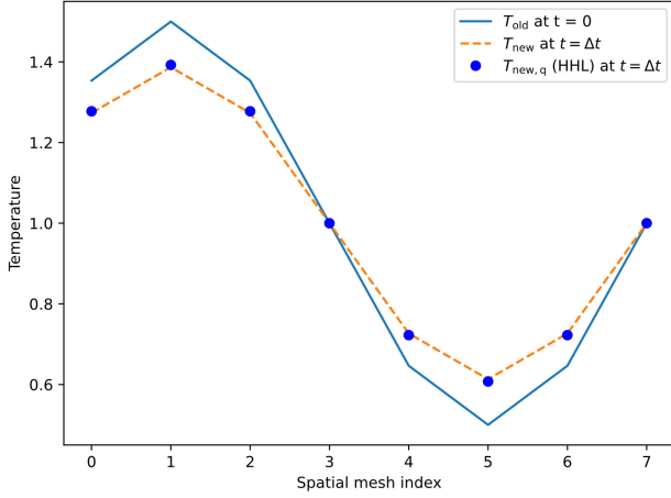
FIGURE 5. One time-step update of the temperature profile according to heat conduction equation by quantum computing (3 qubits) by HHL algorithm. The blue line is the initial temperature profile (with mean equal to 1), the orange dashed line is the new temperature profile at time \Delta t , computed by finite-difference method. The blue dots are the mesh node temperatures computed by the HHL algorithm (ideal statevector simulator). The circuit implementing HHL algorithm with n = 3 input qubits, n_c = 5 clock qubits and 1 ancilla qubit is shown in Fig. 1. In particular, the eigenvalue inversion module with n_c = 5 qubits in the clock register is shown in Fig. 3.
