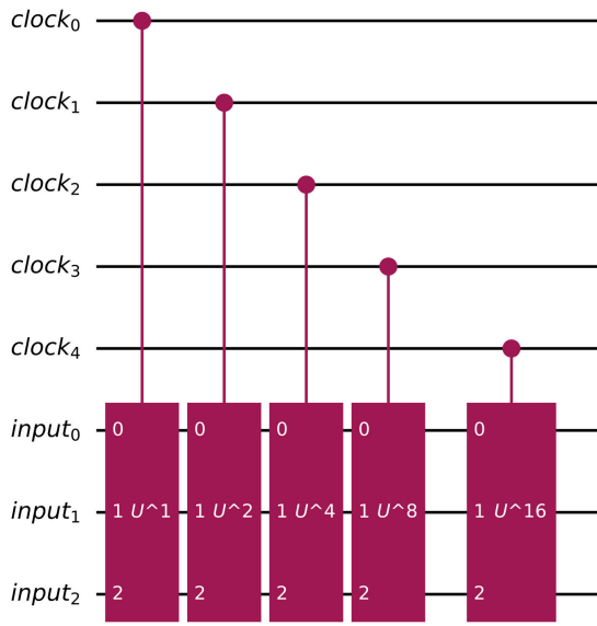
FIGURE 2. Circuit implementing controlled exponentiation (or controlled Hamiltonian evolution) in the HHL algorithm with n = 3 input qubits for solving the same problem discussed in the previous sections and n_c = 5 clock qubits. This circuit shows what is inside the block called “C-exp” in Fig. 1.
