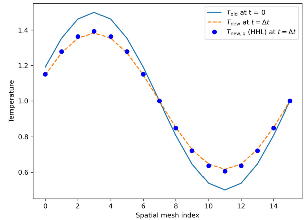
FIGURE 10. One time-step update of the temperature profile according to heat conduction equation by quantum computing by HHL algorithm: n = 4 input qubits, n_c = 8 clock qubits and 1 ancilla qubit. The meaning of the lines and dots is reported in the caption of Fig. 5.
