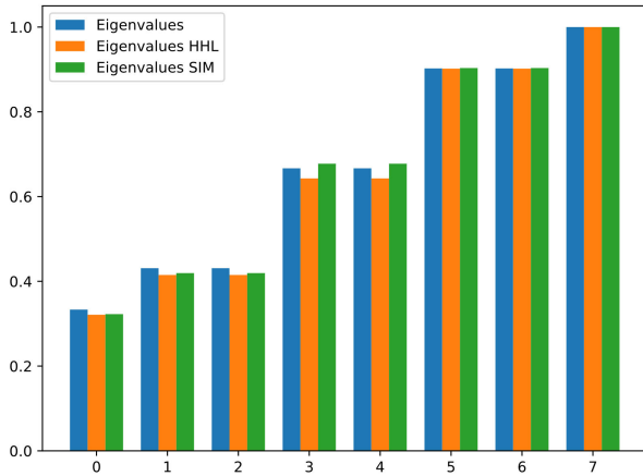
FIGURE 7. Comparison among eigenvalues: (i) original ones for the considered example; (ii) those approximated by the HHL algorithm; (iii) those computed by mimicking the HHL algorithm, but assuming the approximation given by Eq. (74). The abscissa represents the index labels ranging from 0 to N - 1 , corresponding to the normalized eigenvalues of the matrix \hat{r} given by Eq. (16) in increasing order. By design, the maximum normalized eigenvalue is equal to one and it is exactly represented by the binary integer \{1\}^{n_c} . The approximated eigenvalues reported with label 5 and 6 differ from the exact values by less than 0.1% and hence the discrepancies are not visible.
