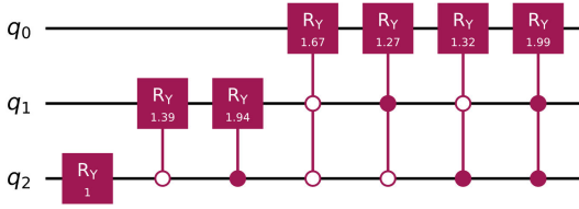
FIGURE 8. Quantum circuit for loading real data in a quantum system state |x\rangle based on a divide-and-conquer algorithm proposed in [24]. Note that the proposed circuit uses only rotations about the Y-axis ( R_Y gates), which are designed by means of a proper binary tree data structure [24]. For clarity, horizontal lines represent quantum wires which correspond to qubits in the circuit, red squares are the R_Y gates (see Eq. (86)), red dots represent control points in controlled gates and empty red circles represent anti-control points (i.e. activated by zero value). The little-endian convention is used [26], meaning that the topmost qubit represents the least significant bit (LSB), while the bottom qubit corresponds to the most significant bit (MSB), which, in this case, forms the trunk of the state tree in the divide-and-conquer strategy [24].
