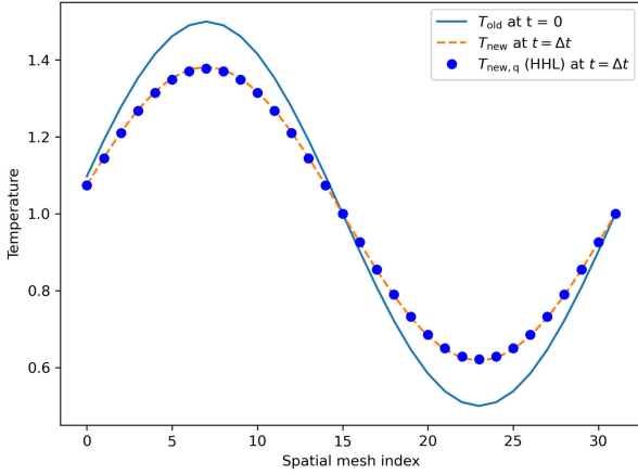
FIGURE 11. One time-step update of the temperature profile according to heat conduction equation by quantum computing by HHL algorithm: n = 5 input qubits, n_c = 10 clock qubits and 1 ancilla qubit. The meaning of the lines and dots is reported in the caption of Fig. 5.
