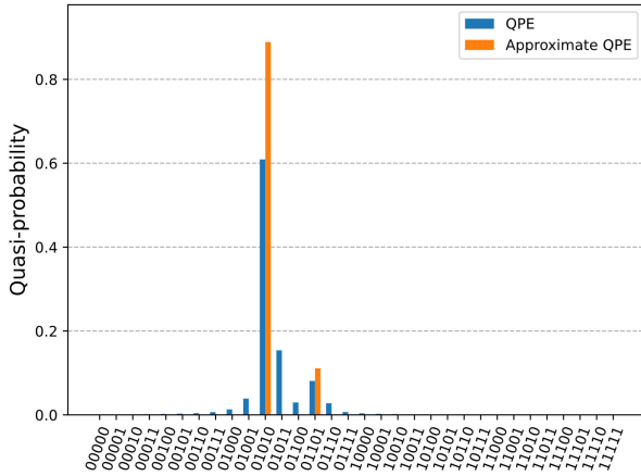
FIGURE 6. Probability distribution of the binarized approximations of the eigenvalues of the problem |k^\lambda\rangle stored in the clock register, after completing QPE. Accessing this information is only possible in ideal (statevector) simulations (otherwise, the wave function would collapse in real computations). The two peaks correspond to (i) eigenvalue k_0^\lambda = 01010 or equivalently (k_0^\lambda)_{(10)} = 10 , and to (ii) eigenvalue k_1^\lambda = 01101 or equivalently (k_1^\lambda)_{(10)} = 13 . It is worth noting that the binarization process implies (k_j^\lambda)_{(10)} \approx (N_c - 1) \lambda_j^\lambda , which introduces some spread in the spectral distribution of the binarized eigenvalues (see Fig. 4).
