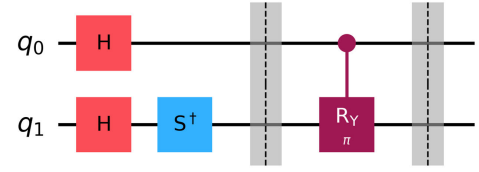
FIGURE 9. Example for explaining the phase kickback phenomenon. For clarity, horizontal lines represent quantum wires which correspond to qubits in the circuit, orange squares are the Hadamard gates H , blue square is the Hermitian adjoint of the phase gate S^\dagger , red square is the R_Y gate (see Eq. (86)) and red dot represents the control point in the controlled gate.
