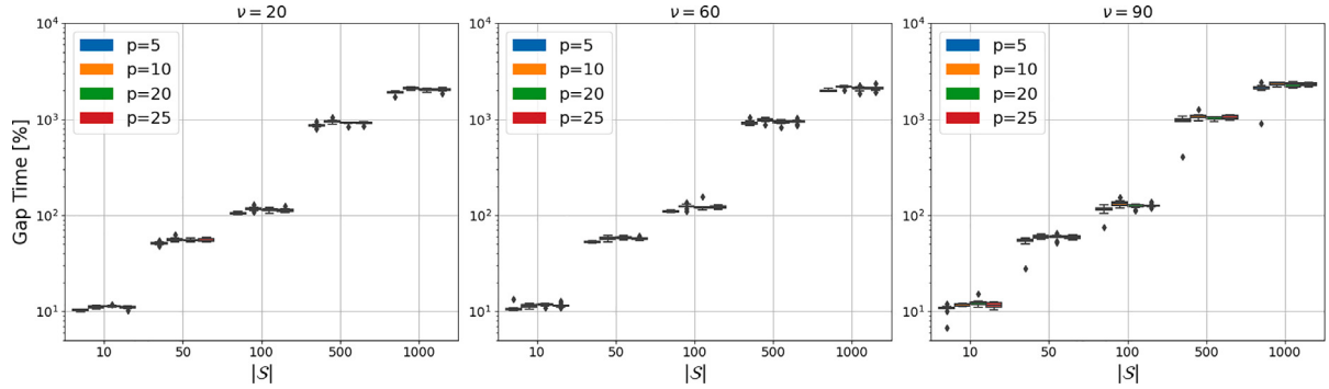
Fig. 8. Computational time gaps for NL instances.
