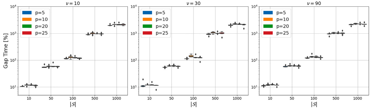
Fig. 7. Computational time gaps for L instances.
