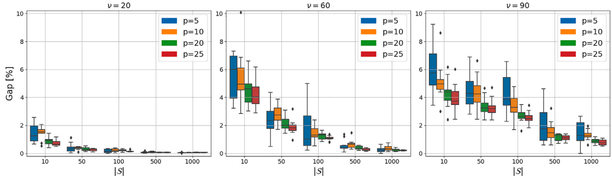
Fig. 6. Percentage optimality gaps for NL instances.
