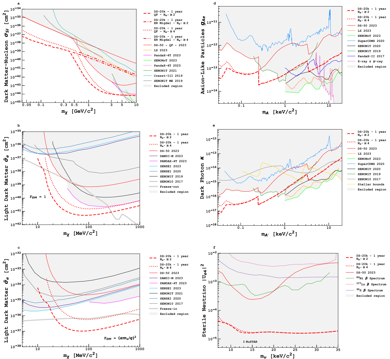
Fig. 4 | Expected DS-20k upper limits at 90% C.L. for various signal models. The x -axis shows the mass of the candidate while the y -axis shows the model parameter. One year of data is assumed. These results (bold red lines, dotted: fit from N_e = 4 , dashed: fit from N_e = 2 ) are compared to the published 90% C.L. limits from DS-50 15,16 , other experiments 7,25–27,50–67 and astrophysical constraints 68–71 , with currently excluded parameter space shaded in light gray. a Spin-independent WIMP–nucleon cross-section when considering the Migdal effect and with quenching fluctuations (QF) for the NR signal. b , c Light dark matter cross-section for an heavy ( b ) and light ( c ) mediator, respectively. Thick lines show cross-sections giving the relic DM
