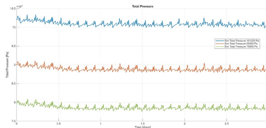
Fig. 5: Total cabin pressure over the mission duration for three different scenarios.
