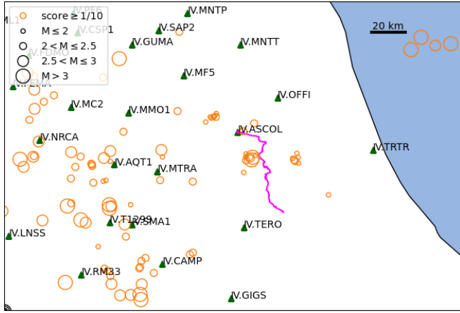
Fig. 2. Map of the cable layout (central Italy), with the location of the closest detected events and closest seismometers of the INGV IV network [46].
