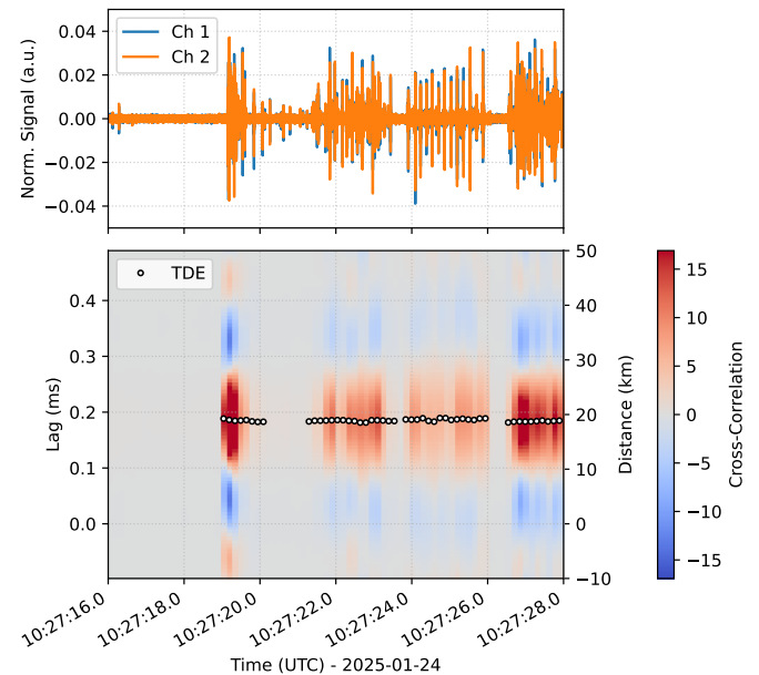
Fig. 7. Localization of tapping events at km 19 of the fiber. Top panel: timeseries (normalized signal) corresponding to recordings at opposite cable ends. Bottom panel: Cross-correlation function vs lag in sliding windows with duration 0.3 s (right y-axis: Lags rescaled to position along the fiber); circles indicate the maximum of cross-correlation for each window, corresponding to the event TDE.
