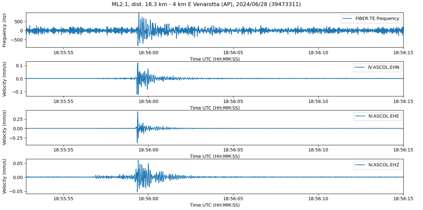
Fig. 3. Timetrace of fiber and the three axes of IV.ASCOL seismometer in occurrence of a magnitude 2.1 event happened 19 km North of the fiber on June 28, 2024. Fiber recordings are shown in terms of the time-derivative of optical phase, i. e. in terms of a frequency shift. IV.ASCOL recordings are obtained from a 3-axes velocimeter; channel codes EHN, EHE and EHZ indicate the North-South, East-West and vertical direction respectively.
