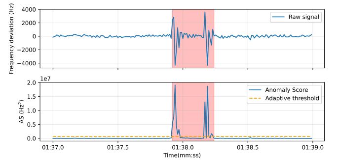
Fig. 5. Top panel: Phase-based timeseries recorded during a vehicle passage on a degraded portion of the road mantle in the fiber proximity. Deformations are plotted in terms of the time-derivative of optical phase, i.e. frequency. Bottom panel: Anomaly Score (AS) and adaptive threshold; the red-shaded region indicates the frame which is recognized as anomalous after merging anomalous samples occurring within a short time.
