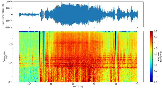
Fig. 4. Perturbation (timeseries and spectrogram) induced by a storm with strong wind gusts on the aerial fiber span. Deformations are plotted in terms of the time-derivative of optical phase, i.e. frequency.
