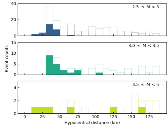
Fig. 1. Detection rate for events of low ( 2.5 \leq M < 3.0 , top panel), mid ( 3.0 \leq M < 3.5 , middle panel) and large ( 3.5 \leq M < 5.0 , bottom panel) magnitude occurred over the period 2022-2025, as a function of their hypocentral distance to the closest point of the fiber. Filled (empty) bars indicate the counts of detected (total) events for each distance.
