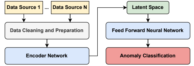
Fig. 1: MERGE’s Architecture Overview
