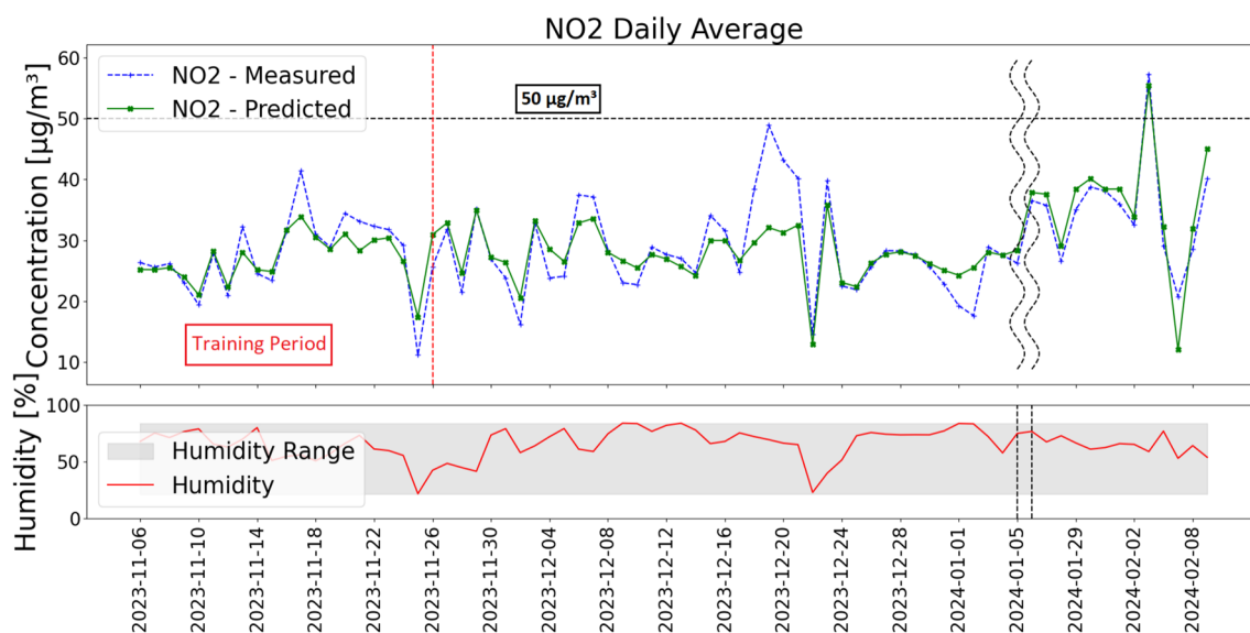
Fig. 13 Comparison of daily average \text{NO}_2 concentrations measured by the reference instrument (dashed blue line) and those estimated by MONICA (green line) using the MLR regression model trained over a three-week period. The regulatory limit established by Directive (EU)
