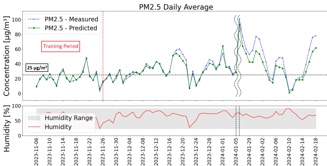
Fig. 11 Comparison of daily average PM_{2.5} concentrations measured by the reference instrument (dashed blue line) and those estimated by MONICA (green line) using the MLR regression model trained over a three-week period. The regulatory limit established by Directive (EU)
