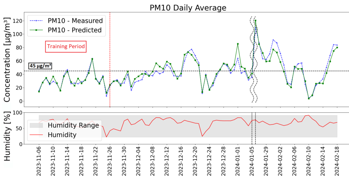
Fig. 12 Comparison of daily average PM_{10} concentrations measured by the reference instrument (dashed blue line) and those estimated by MONICA (green line) using the MLR regression model trained over a three-week period. The regulatory limit established by Directive (EU)
