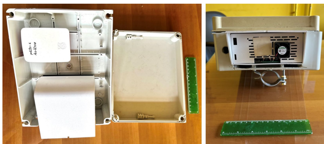
Fig. 1 ENEA MONICA device. Left: Internal view of the device. Right: Close-up of the chamber housing the PM and \text{NO}_2 microsensors. The overall dimensions of the device are 19 \times 24 \times 10 \text{ cm}^3 , and
