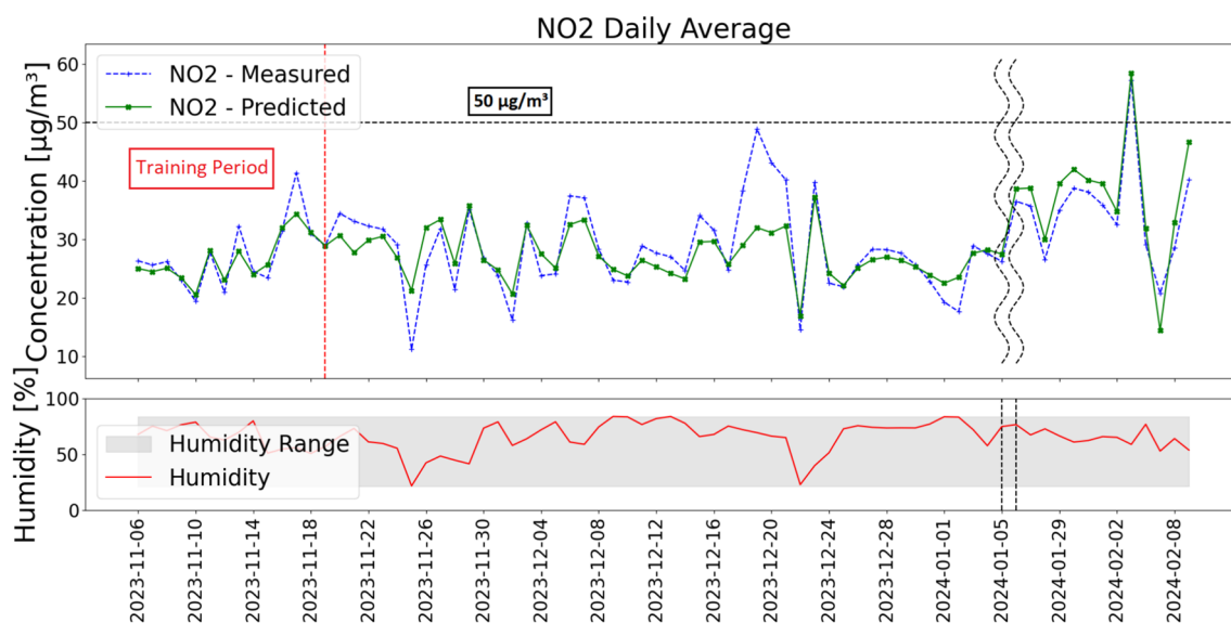
Fig. 10 Comparison of daily average \text{NO}_2 concentrations measured by the reference instrument (dashed blue line) and those estimated by MONICA (green line) using the MLR regression model trained over a two-week period. The regulatory limit established by Directive (EU)
