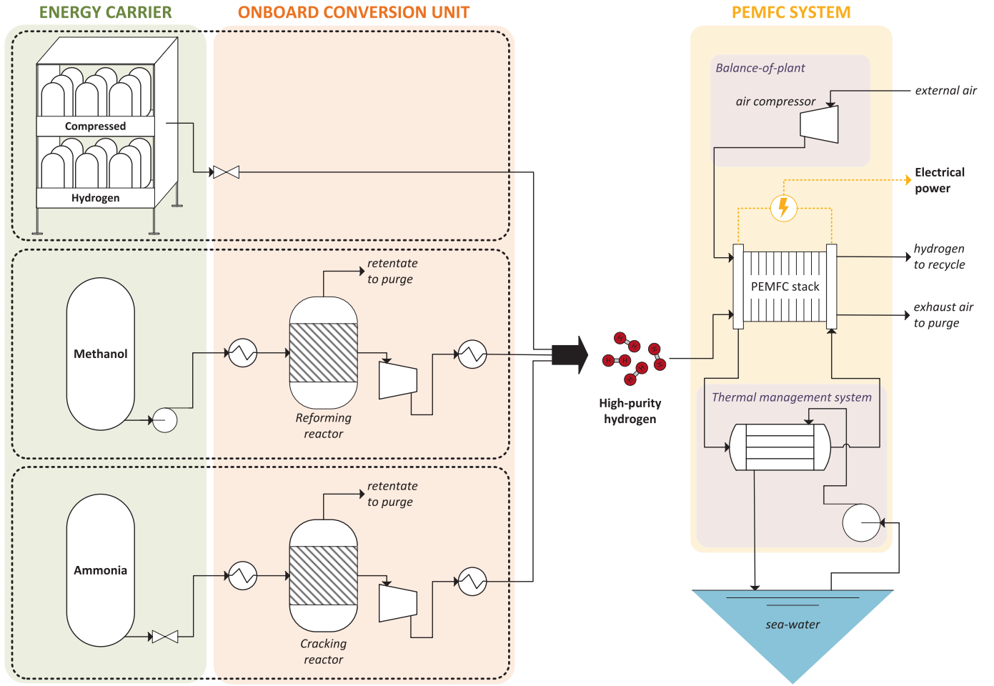
Fig. 2. Process scheme of the electrified system, accounting for three different storage methods, including compressed hydrogen, methanol and ammonia, the conversion units to release pure hydrogen, and the PEMFC system, with seawater cooled liquid-based thermal management system.
