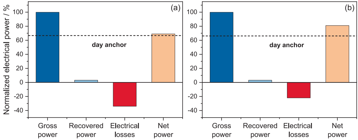
Fig. 7. Electric power distribution for methanol-based system, normalized to the PEMFC gross power output, in the case of (a) air-cooled liquid-based TMS and (b) seawater-cooled liquid-based TMS.
