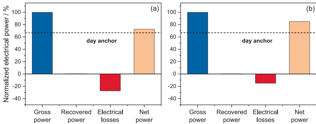
Fig. 9. Electric power distribution for ammonia-based system, normalized to the PEMFC gross power output, in the case of (a) air-cooled liquid-based TMS and (b) seawater-cooled liquid-based TMS.
