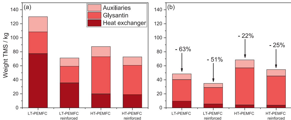
Fig. 10. Comparison of TMS component weights for methanol-based system with different PEMFC technologies, in the case of (a) air-cooled liquid-based TMS and (b) seawater-cooled liquid-based TMS.
