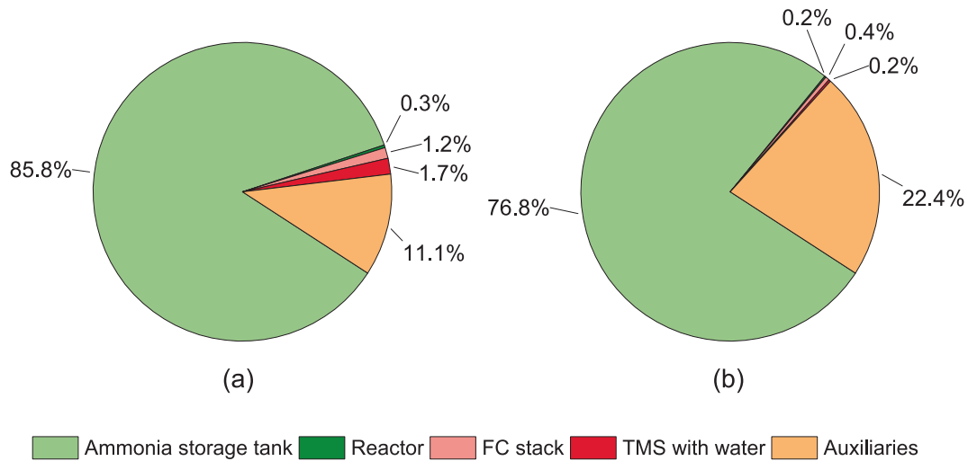
Fig. 8. Ammonia-based system: Distribution of weight (a) and volume (b) of ammonia-based system with baseline LT-PEMFC and seawater-cooled, liquid-based TMS.
