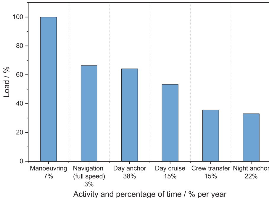
Fig. 1. 35–45 m yacht load distribution for hoteling purpose normalized to the maximum power demand, and operation time distribution over a year. Bars represent normalized power demand, while percentages below each bar indicate the fraction of operating time.
