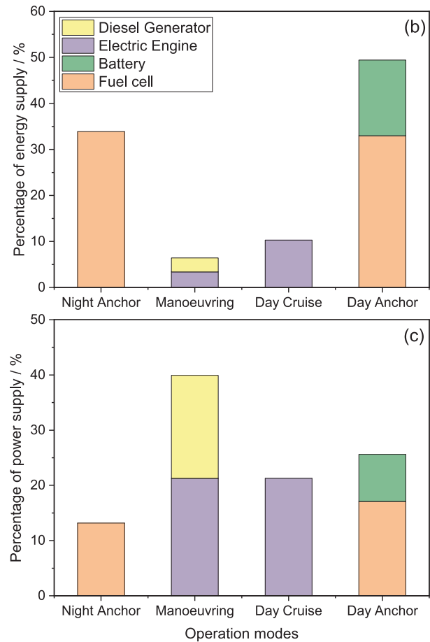
Fig. 5. (a) Simplified scheme of energy allocation among the components of the hybrid system across different operational modes for hoteling requirements; (b) energy distribution percentage and (c) power supply percentage for the same modes in a 35–45 m yacht.
