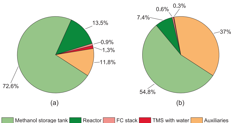
Fig. 6. Methanol-based system: Distribution of weight (a) and volume (b) of methanol-based system with baseline LT-PEMFC and seawater-cooled, liquid-based TMS.
