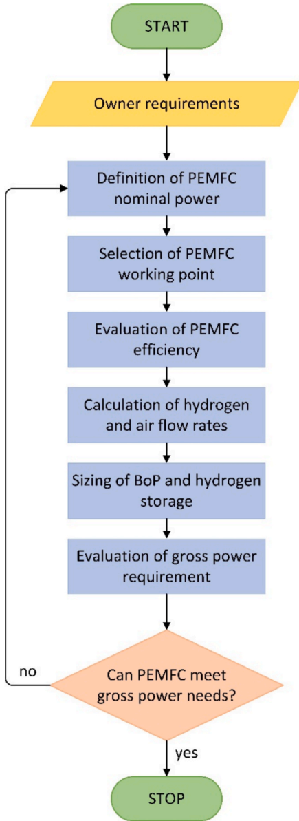
Fig. 3. Flow diagram of calculation procedure for PEMFC sizing.
