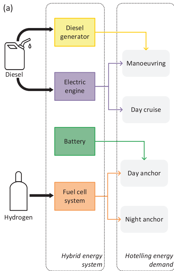
Fig. 5. (a) Simplified scheme of energy allocation among the components of the hybrid system across different operational modes for hoteling requirements; (b) energy distribution percentage and (c) power supply percentage for the same modes in a 35–45 m yacht.
