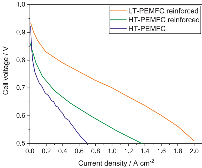
Fig. 4. Polarization curves of the different PEMFC used in the analysis [41–43].
