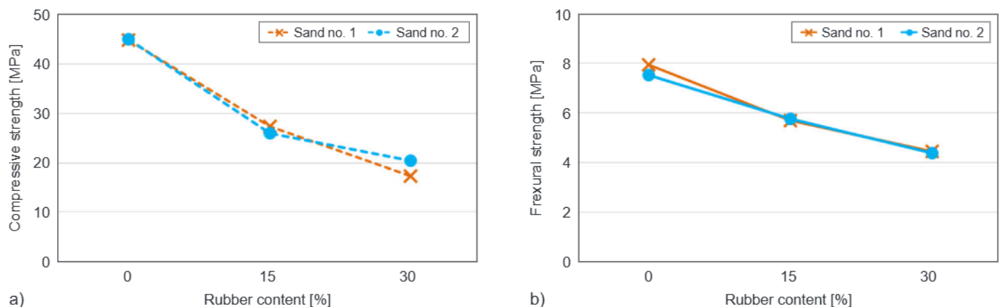
Fig. 5. The mechanical properties of mortars after 28 days of curing: a) compressive strength, b) flexural strength
