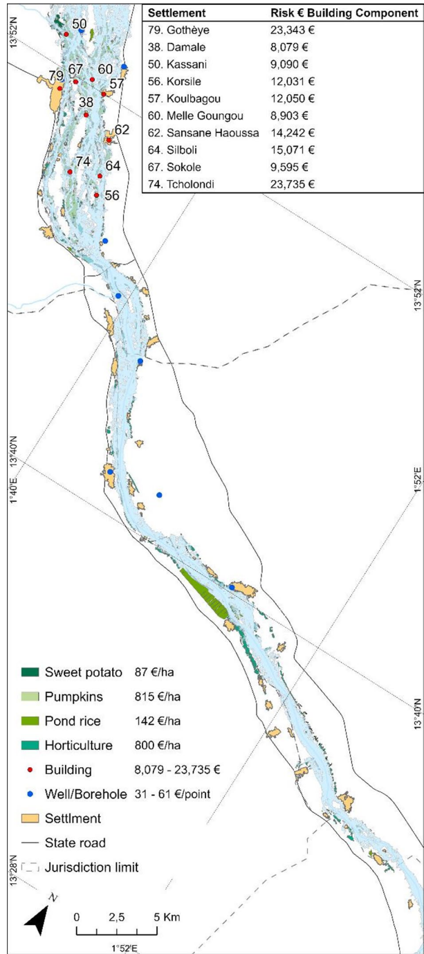
Fig. 12 Risk for Guinean floods with 10-year RP
