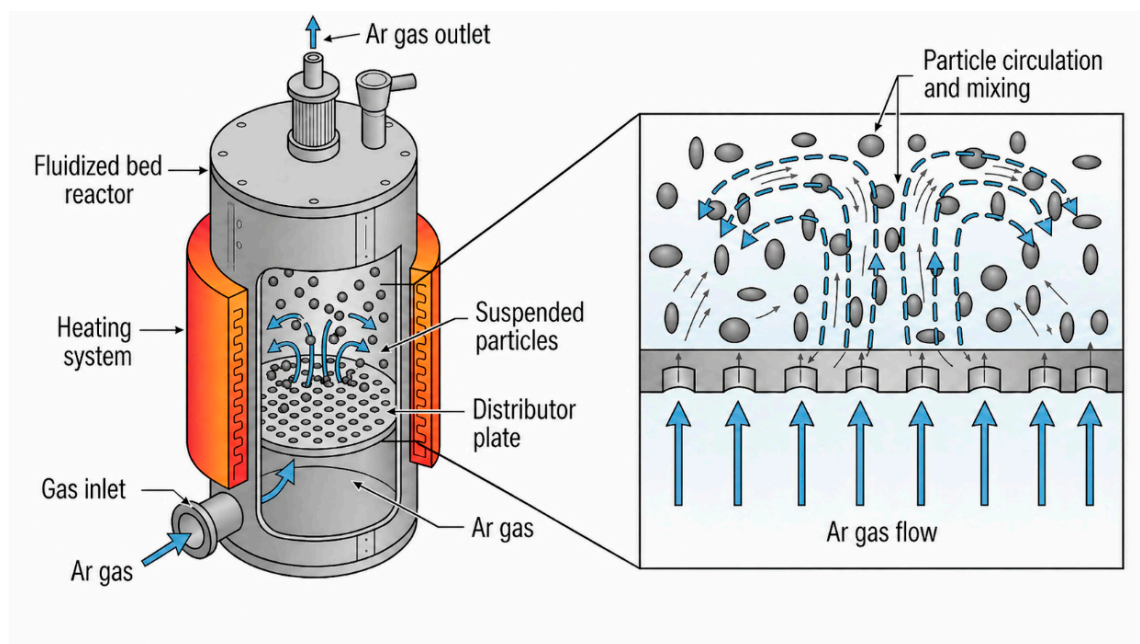
Figure 7. Schematic illustration of fluidized-bed-assisted powder classification and fine-particle removal.
