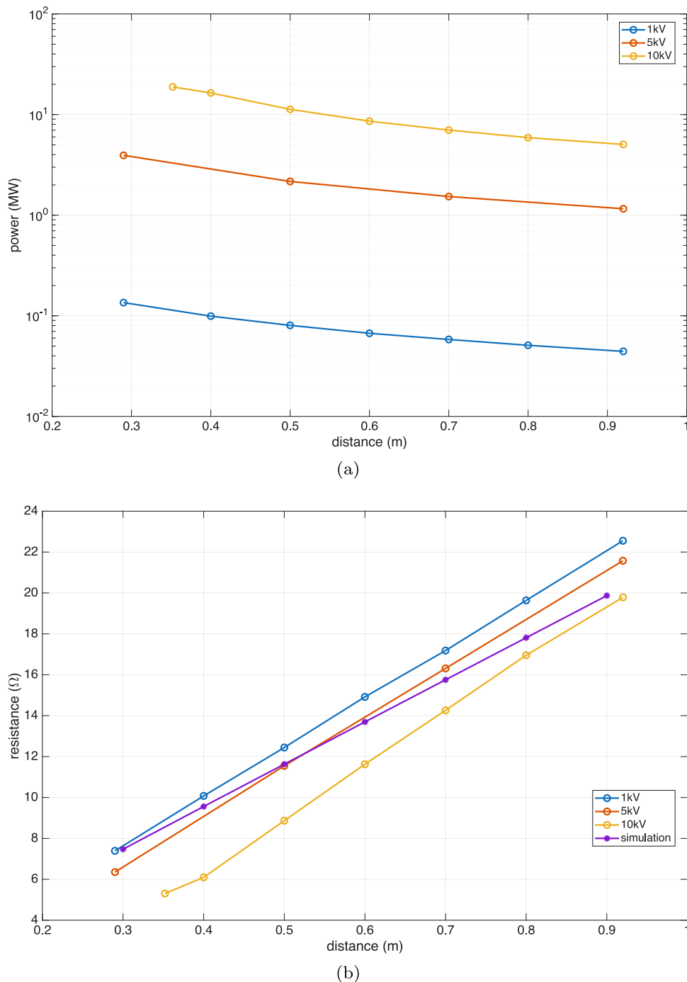
FIGURE 5 | Testing of the refurbished solution at different voltage levels: (a) measured power versus electrode distance, (b) measured equivalent resistance versus electrode distance. The simulated curve in (b) refers to the numerical model described in Section 5.2 and discussed in Section 5.3.
