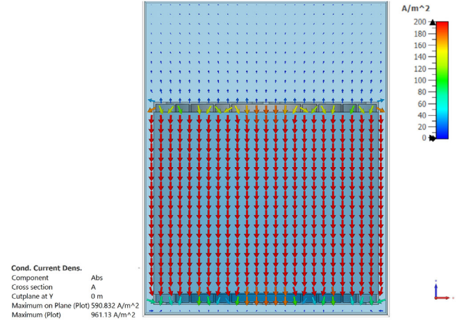
FIGURE 9 | Current density (range 0–200 A/m²) with maximum electrode distance (0.9 m).
