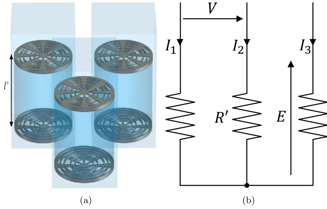
FIGURE 4 | (a) Sketch of the refurbished dump-load system, (b) equivalent circuit.
