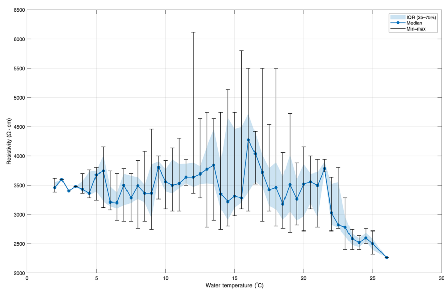
FIGURE A2 | Po River water resistivity as a function of temperature (digitized dataset from Figure A1). The median is shown with filled markers, the shaded band indicates the interquartile range (25% – 75%), and whiskers report the minimum and maximum values in each temperature interval.
