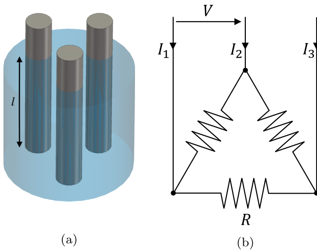
FIGURE 2 | (a) Sketch of the original dump-load system, (b) equivalent circuit
