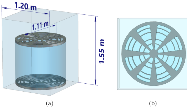
FIGURE 7 | Refurbished configuration: (a) geometry, (b) detail of the electrode (top view).
