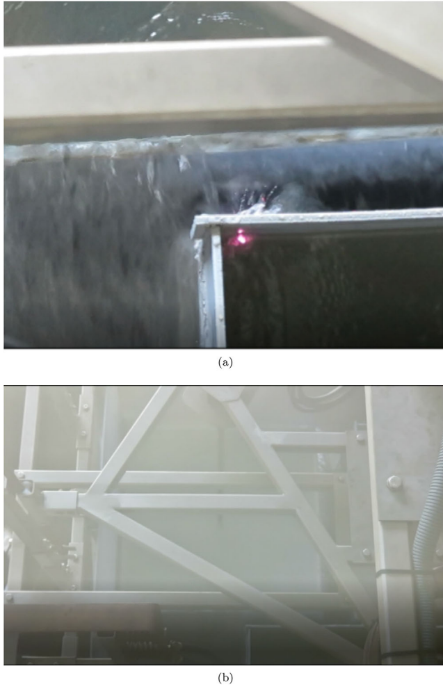
FIGURE 6 | (a) Electrical sparks between the spilling water and the tank of another phase, (b) steam formation at rated power.
