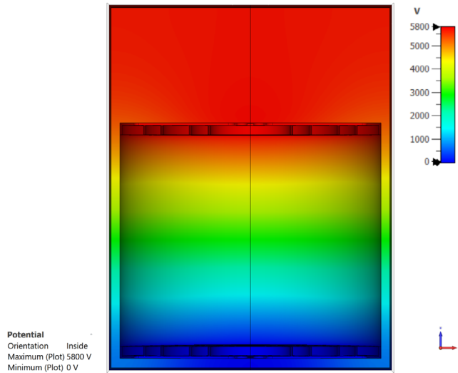
FIGURE 8 | Electrical potential (range 0–5.8 kV) with maximum electrode distance (0.9 m).
