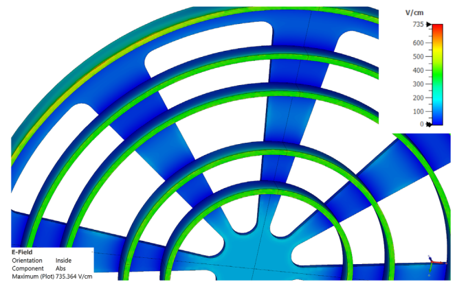
FIGURE 10 | Simulated electric field distribution on the upper electrode surface at a 30 cm spacing.
