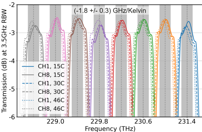
Fig. 18. AWG transmission spectra measured at 15°C, 30°C and 46°C. RBW set to 3.5 GHz.
