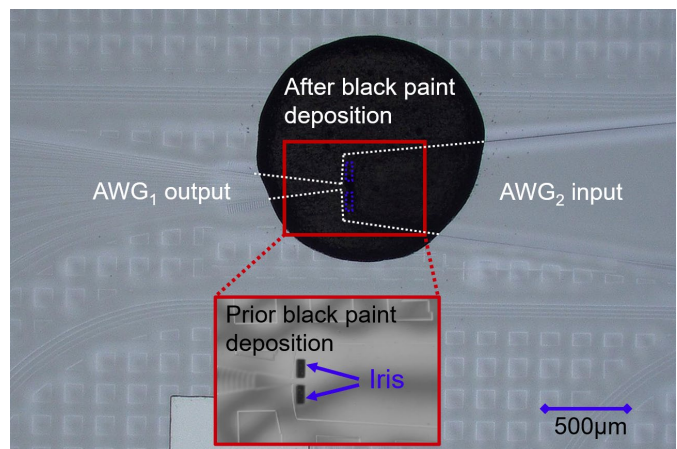
Fig. 10. To reduce crosstalk between channels, an iris is created at the location where the first and second AWG meet (white dashed lines). The iris is realized by etching a slot which is subsequently filled with black paint.
