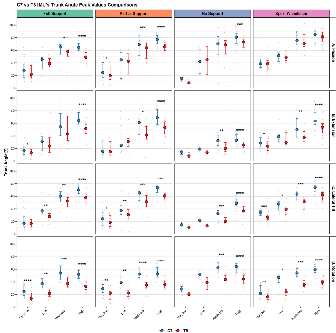
Figure 6. Comparison of trunk angle peak values measured by C7 and T8 IMUs across four ergonomic conditions and four Trunk Function Groups. All values are expressed as positive values. Blue and red filled circles (black outlines) represent median values for C7 and T8 measurements, respectively; error bars indicate the interquartile range. Semi-transparent points show individual participant data. Panel rows represent movement directions (A–D); columns represent ergonomic conditions. Wilcoxon Signed-Rank Test (* p < 0.05 , ** p < 0.01 , *** p < 0.001 , **** p < 0.0001 ).
