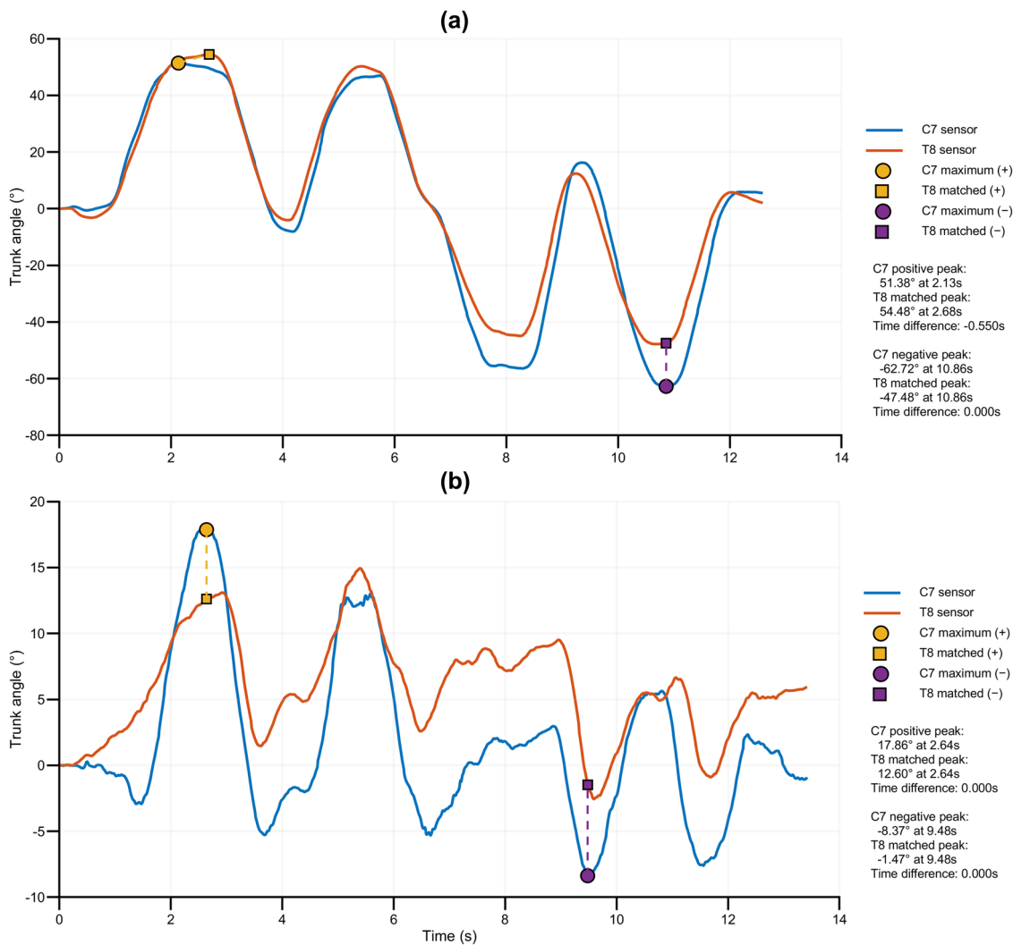
Figure 3. Representative examples of the peak matching procedure during lateral tilt in the partial support condition. Panel (a) shows a participant with lower limb impairment but fully preserved trunk function (WB Class 4.5). Panel (b) shows a participant with minimal trunk function (WB Class 1.0) demonstrating a limited volume of action (VoA) with visible compensatory upper trunk movements. Both graphs display lateral tilt cycles with positive peaks indicating left lateral tilt and negative peaks indicating right lateral tilt, interspersed with returns to neutral position (approximately 0^\circ ). Yellow circles indicate C7 peaks matched to corresponding T8 peaks (yellow squares). Purple markers indicate negative peaks (right lateral tilt).
