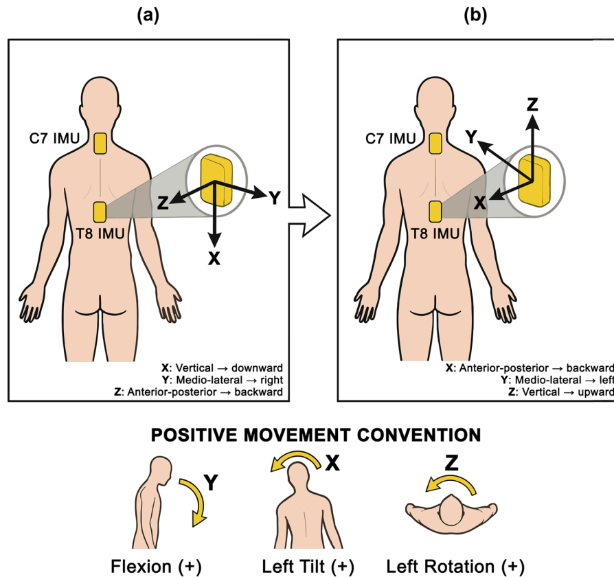
Figure 2. IMU Sensor orientation processing flow: (a) Sensors were placed at C7 and T8 vertebrae with initial coordinate axes: x-vertical (inferior), y-medio-lateral (right), z-antero-posterior (posterior). (b) Sensor orientations were rotated to align the x-axis with gravity during baseline trials, then transformed using rotational matrices to establish the anatomical reference frame: Z-vertical (upward), Y-medio-lateral (left), and X-antero-posterior (backward). This standardisation defined flexion, left tilt, and left rotation as positive angular values.
