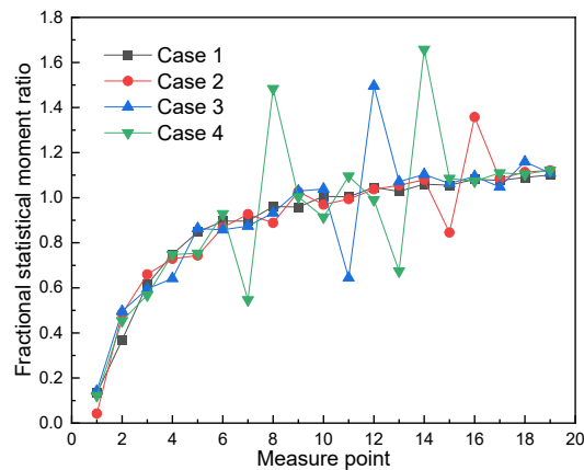
(c) 30dB
