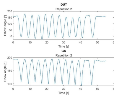
Figure 6: Comparison between the waveform of the elbow angle during repeated flexion-extensions recorded by the device under test (DUT) - the DEHUR system, and the Wearnotch system.
