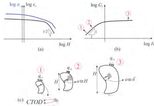
Fig. 18. Scaling laws derived from the dimensional analysis of the BPD model parameters. (a) Tensile strength and critical strain and (b) fracture energy. (c) Schematic representation of the fracture energy scaling law (adapted from [30]).
