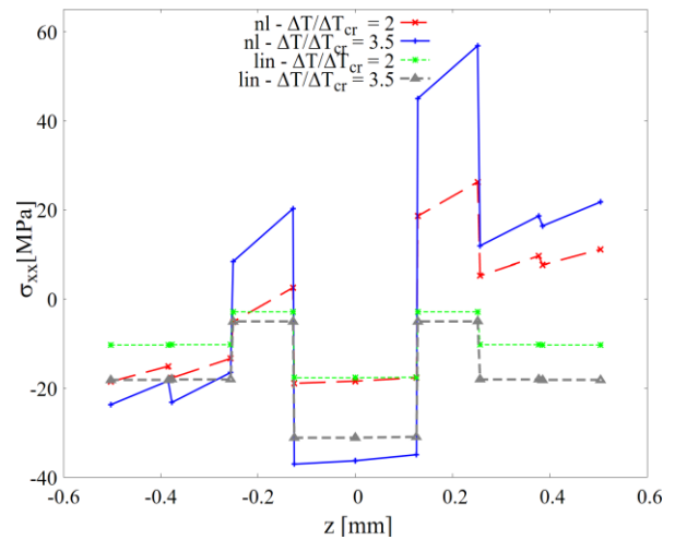
Figure 4: In plane normal stress with different loads. 10 \times 10 Q9 and LE2 in-thickness expansion. Comparison between linear and non-linear analyses.
