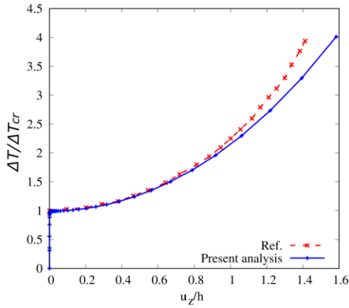
Figure 2: z-displacement and overtemperature graph with non-dimensional value. Reference results from [10].
