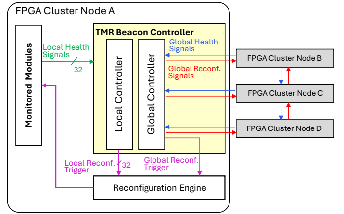
Fig. 1 The developed Beacon Controller architecture.
