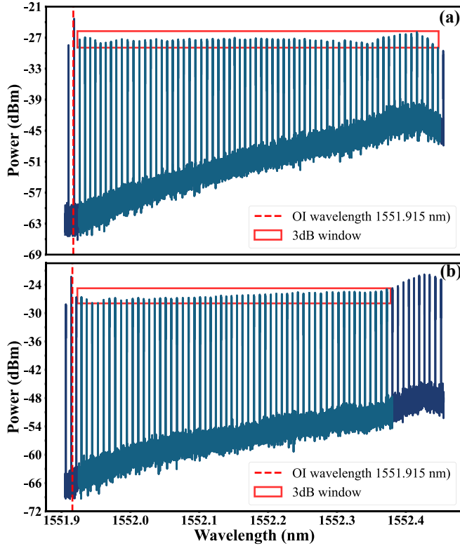
Fig. 2. A close-up view of the optical spectra of the generated OFCs. (a) OFC 1 with the 3-dB window ranging from 1551.920 nm to 1552.455 nm and (b) OFC 2 with the 3-dB window ranging from 1551.920 nm to 1552.350 nm.
