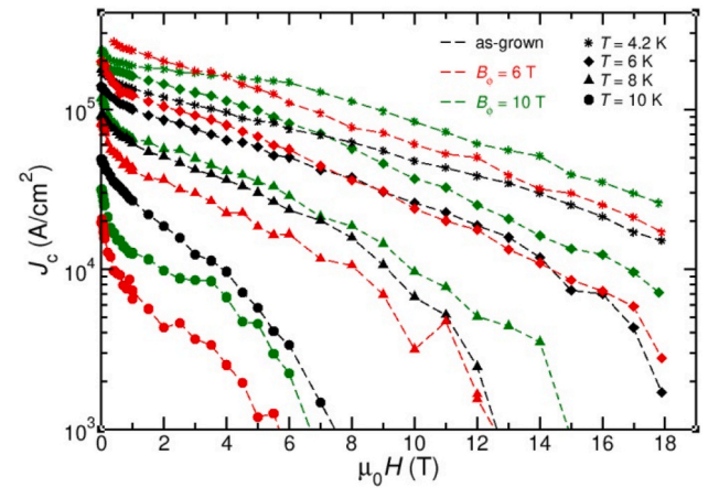
Fig. 5. In-field behavior, up to 18 T, of J_c for the investigated strips at different temperatures in the range 4.2 – 10 K (see symbol legend). J_c curves achieved on the as-grown strip are plotted in black, while the red and green curves refer to J_c values obtained on the irradiated strip at the dose equivalent fields, B_\phi = 6 and 10 T, respectively.
