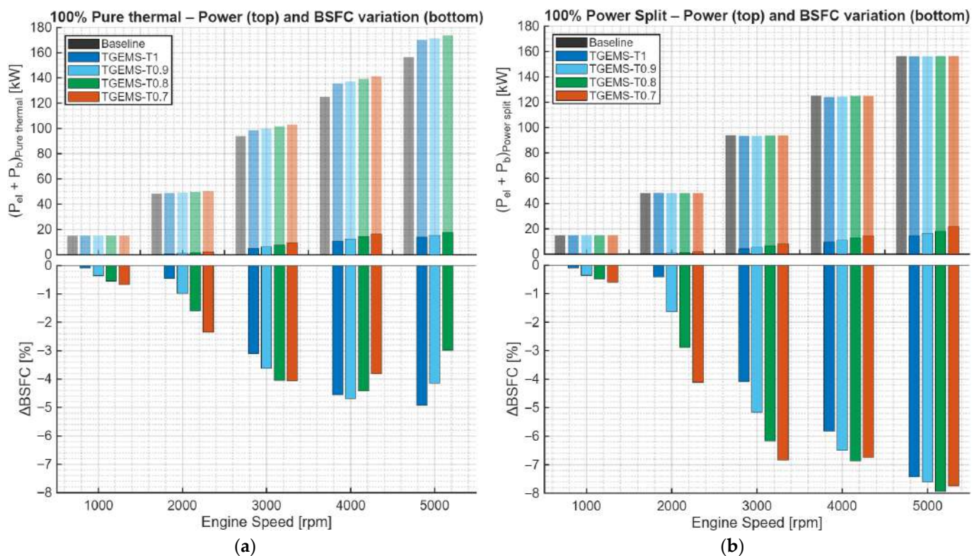
Figure 16. P_{b,tot} and \Delta bsfc variation in function of T-stage dimension in 100% loading condition (baseline bmep ) with different energy management strategies and P_{b,tot} explicit components ( P_{el} solid and P_b transparent): (a) 100% Pure Thermal, (b) 100% Power-Split.
