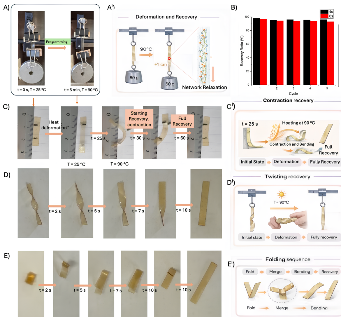
Figure 7. Shape memory behavior of a thin 4s film: (A) stretching under load; (B) recovery ratio as a function of the number of cycles; (C) U-shaped bending; (D) twisting; and (E) folding. The corresponding schematic representations are displayed in A', C', D', and E'.
