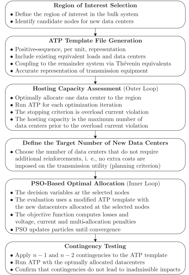
Fig. 4. Block diagram of the proposed methodology.
