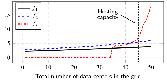
Fig. 6. Objective function components' behavior during hosting capacity assessment ( f_1 given in pu; f_2 and f_3 are dimensionless).
