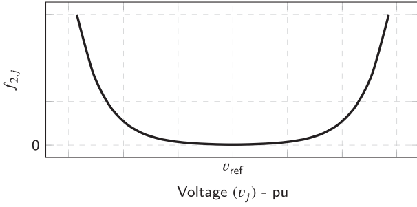
Fig. 2. Individual node voltage violation penalty.
