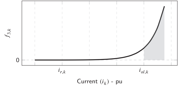
Fig. 3. Individual branch current violation penalty.
