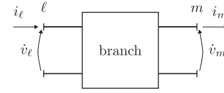
Fig. 1. Complex power per branch.
