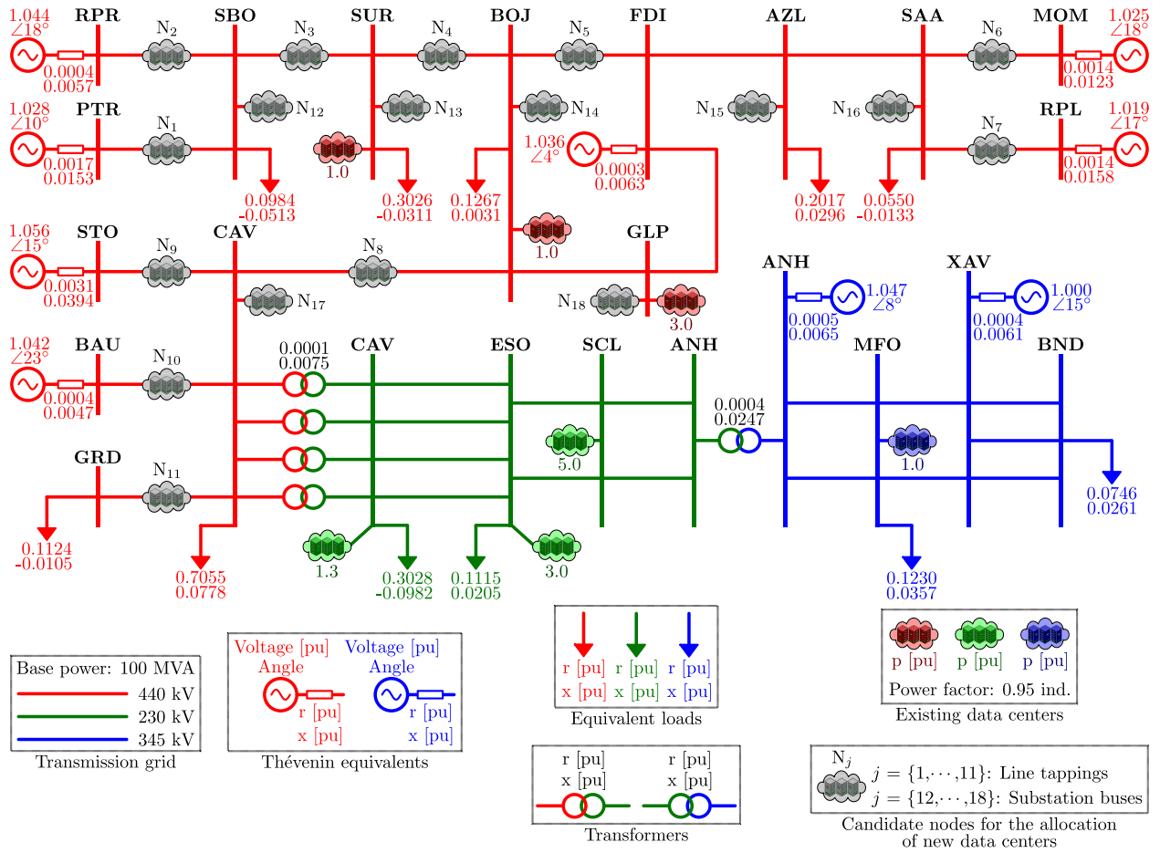
Fig. 5. Transmission grid considered in this case study, with eighteen candidate nodes for the allocation of new data centers.
