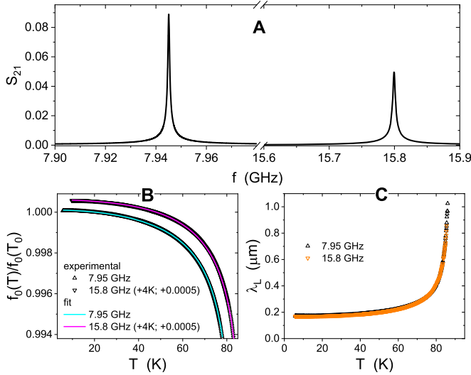
Fig. 1. (A) CPWR resonance curves (magnitude of S_{21} vs. frequency) at T = 5.8 K for the fundamental (left) and the first harmonic mode (right). (B) Examples of the normalized resonance frequency fit. The first harmonic curves at 15.8 GHz were shifted by 4 K horizontal and 0.0005 vertical, for the sake of clarity. (C) London penetration depth as a function of temperature, obtained by fitting data for both the fundamental and first harmonic modes.
