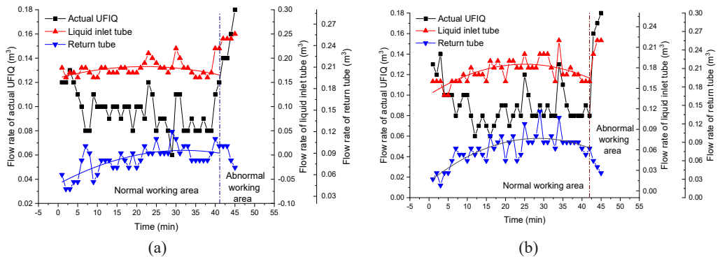
Fig. 11. Curve diagram of unit flow rate variation of 1~2 # fracturing holes during HF. (a) 1 # fracturing holes; (b) 2 # fracturing holes
