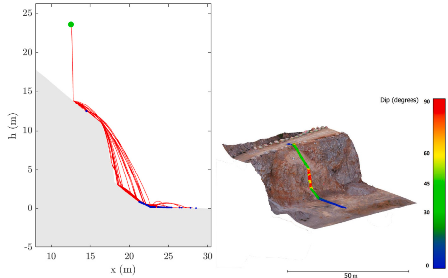
Fig. 7. Simulated trajectories for Site 4. Only one block release is shown, and the plotted trajectories correspond to the fragments generated during impact. The release point is shown in green, fragment trajectories in red, and end points in blue. The grey area represents the slope profile. The right sketch illustrates a 3D view of the slope, from Gili et al. 13
