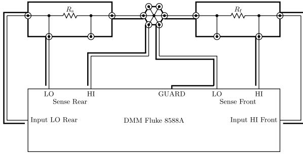
Fig. 11. Resistance ratio measurement schematic; the DMM measures the ratio between two 10 kΩ four-terminal resistance standards R_f and R_s in “True ohm” mode. The DMM injects a 100 \mu\text{A} current between the terminals Input LO Rear and Input HI Front, which is reversed periodically. R_f/R_s is measured as the ratio between the voltage V_{R_f} across R_f and the voltage V_{R_s} across R_s .
