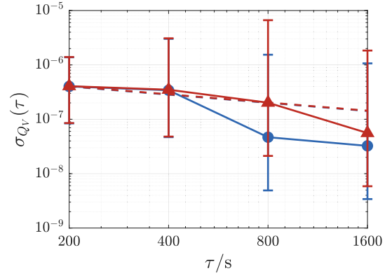
Fig. 12. Allan deviation for an example measurement of the voltage ratio measurements Q_V : the blue filled circles represent the measurements relative to the forward configuration; the red filled triangles represent the measurements relative to the reverse configuration. The dashed lines represent the theoretical Allan deviation of a white noise.
