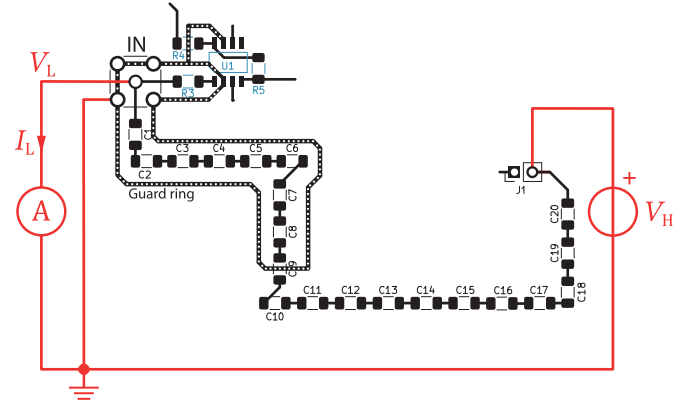
Fig. 8. PCB signal-layer detail of interest for the measurement of r . Interconnections and soldered components are represented in black; unsoldered components, in blue. The red schematic shows the source-measure unit connection: V_H is applied to the right pin of J_1 , I_L is measured from the inner conductor of the IN SMA, and the outer conductor is connected to ground. The picture also shows the guard ring encircling the IN center conductor, the inverting, and non-inverting inputs of U_1 and C_1 – C_9 .
