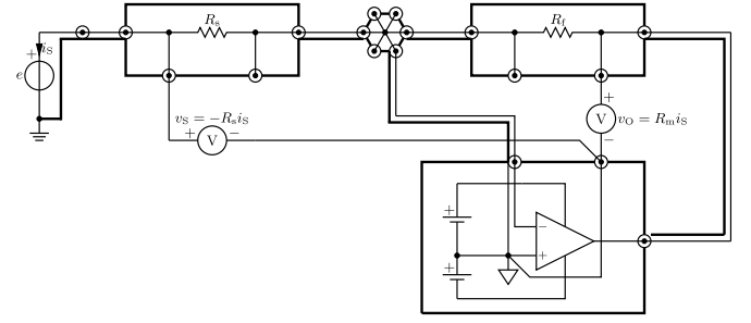
Fig. 10. Voltage ratio measurement configuration: the transresistance R_m \approx R_f of the TRA multiplies the input current i_s , generated by a voltage e = \pm 1 V applied through a resistance R_s . The feedback resistance R_f and R_s are two 10 k \Omega four-terminal resistance standards. The DMM measures the ratio between the output voltage v_O and the voltage v_s across R_s .
