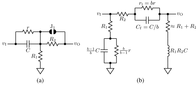
Fig. 5. (a) Principle schematic of the compensation T network: the capacitance C has leakage resistance r ; R_1 and R_2 compose a voltage divider; and the jumper J_1 allows to short R_2 . (b) Equivalent schematic of the network (a) with equivalent impedances between the input and output nodes and the ground. The compensation impedance between the input and the output of TRA is R_2 + (br) \parallel (b/(sC)) with b = (R_1 + R_2)/R_1 (when J_1 is shorted, R_2 = 0 and b = 1 ).
