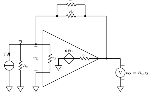
Fig. 2. TRA DC model for gain error evaluation. C_f has been substituted by the leakage resistance r_l and the op amp by an equivalent model with open-loop gain a , differential resistance r_d , and output resistance r_o .
