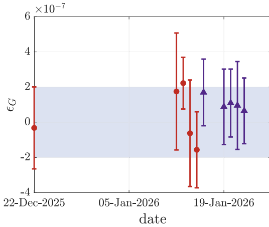
Fig. 14. Gain error \epsilon_G measurement over time: the red filled circles are measurements taken without temperature control on the four-terminal resistors; the purple triangles are measurements taken with temperature-controlled resistors. The blue shaded region is the target accuracy of the amplifier.
