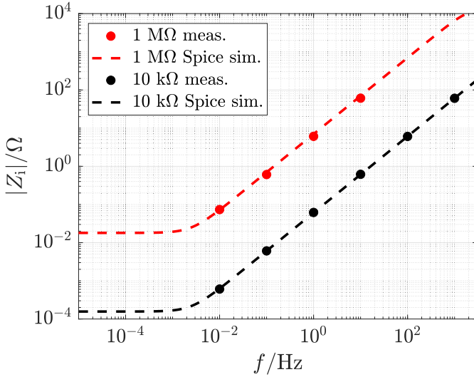
Fig. 9. Measurements of the input impedance modulus |Z_i| as a function of the frequency f for R_f = 10 k \Omega (black markers) and R_f = 1 M \Omega (red markers), together with the corresponding SPICE simulations (dashed lines).
