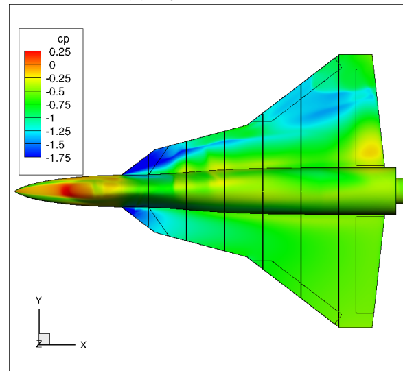
(b) RANS
