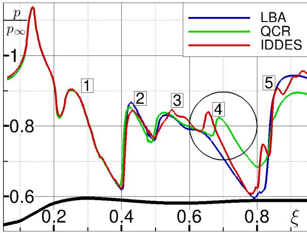
Figure 4: Shock wave locations on the aircraft fuselage. Black line indicates aircraft geometry.
