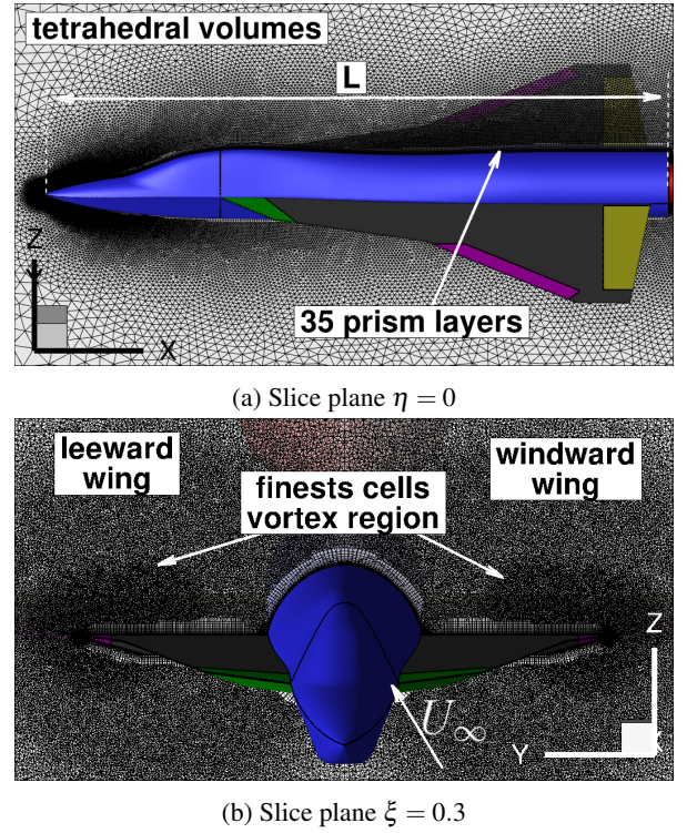
Figure 1: ADS-NA2-W1 geometry and mesh.
