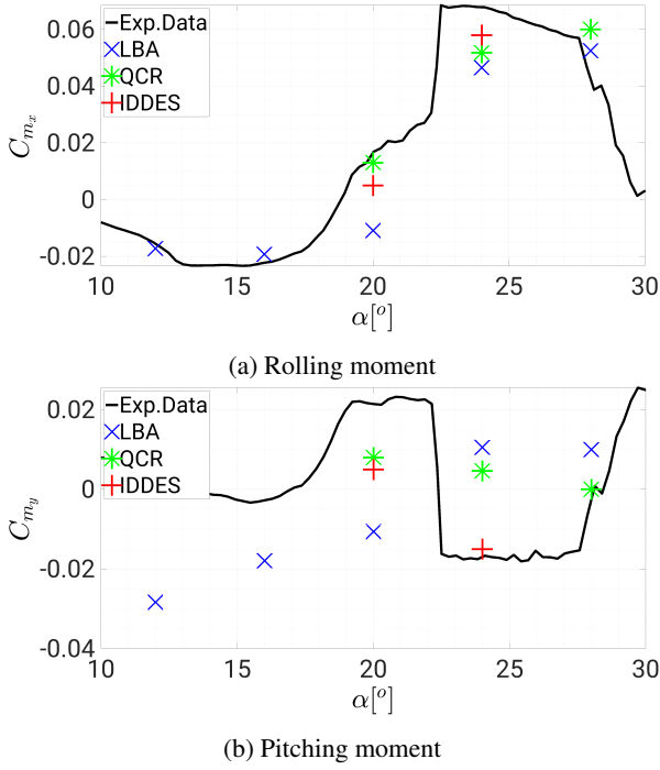
Figure 2: Aerodynamic coefficients over angle of attack with Ma = 0.85 , Re = 12.53 \cdot 10^6 and \beta = 5^\circ .
