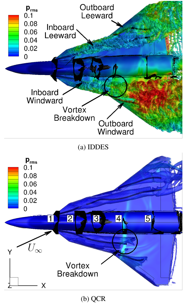
Figure 3: Rms pressure normalized by free-stream pressure p_{rms}/p_\infty and Q-criterion iso-surface, IDDES and QCR results for \alpha = 20^\circ and \beta = 5^\circ . Black: isosurface of Ma = 1 and vortex center lines.
