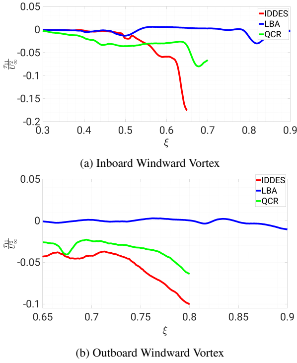
Figure 7: Numerical evolution of the normalized specific Reynolds stress \tau_{11}/U_\infty in the leading-edge vortex core.
