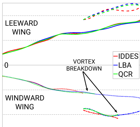
Figure 5: Vortex core line.
