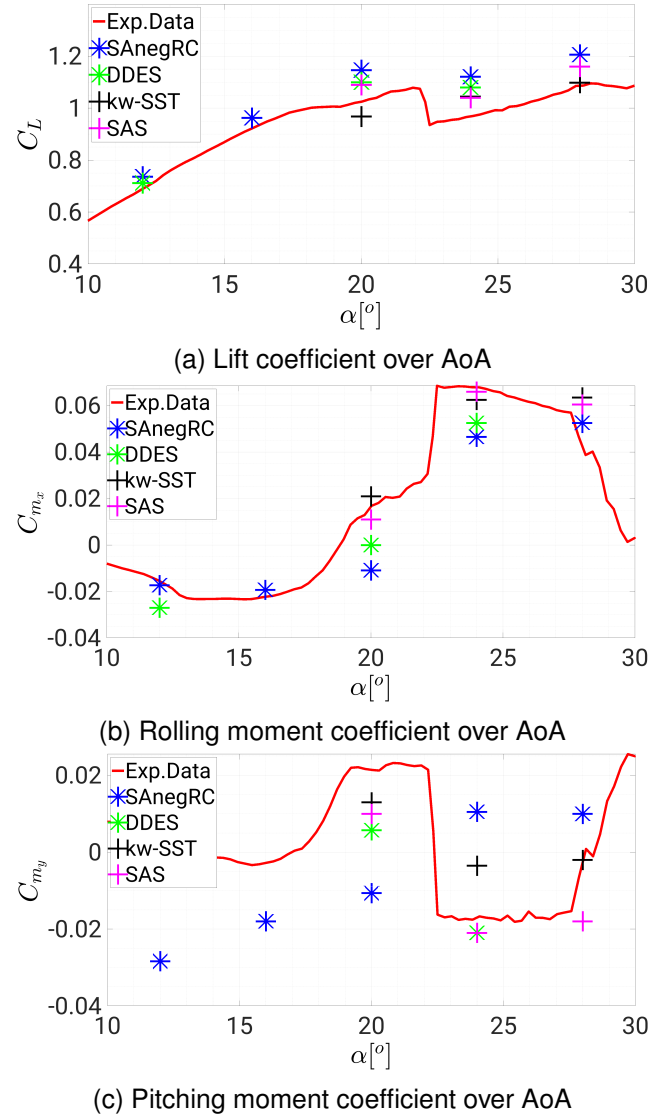
Figure 2 – Polar plots, comparison between experimental and numerical data with Ma_\infty = 0.85 , Re_\infty = 12.53 \cdot 10^6 and \beta = 5^\circ
