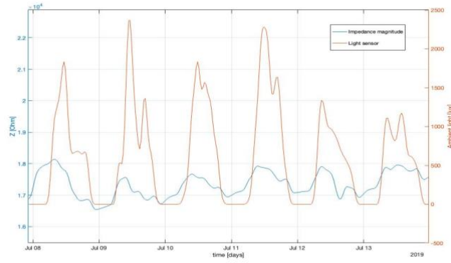
Figure 15: Tobacco plant signal across time
