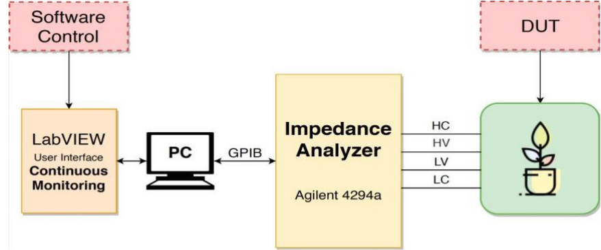
Figure 5: Impedance measurement setup schematic diagram including the plant connected and the control system designed
