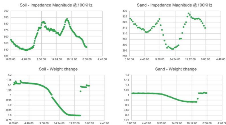
Figure 18: Soil vs sand behavior
