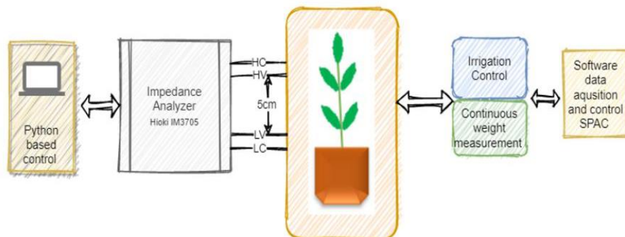
Figure 9: Outdoor impedance monitoring setup schematics
