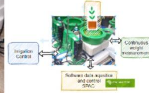
Figure 16: left: Continuous monitoring of a tobacco plant in the TAU greenhouse; right: schematic description of the monitoring system
