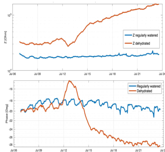
Figure 14: Impedance measured across time of 2 tomato plants, the one regularly watered and the other dehydrated, both impedance magnitude (top) and phase (bottom) present response to regular hydration vs dehydration.
