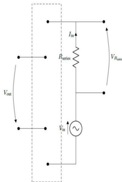
Figure 4: Schematic of a manual impedance measurement setup
