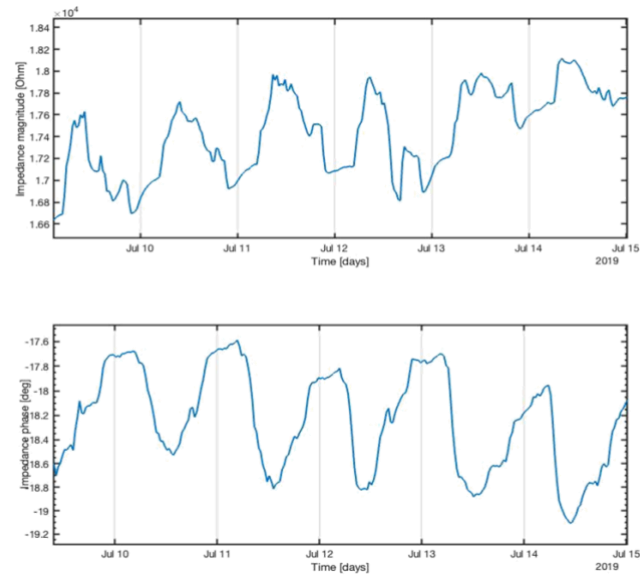
Figure 13: Impedance measurement shown at the centroid frequency across six days. The plant was manually watered once a day. The Impedance magnitude (top) and phase (bottom) are shown separately across time. Both measures show a repetitive behavior across the different days, indicating that the impedance data may follow the plant's daily cycle trend.
