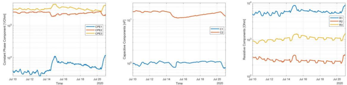
Figure 22: Lumped element circuit parameters across time. A: the insert: The plan physically based lumped electrical model, B: the constant phase elements
