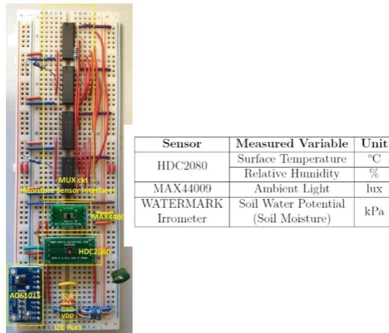
Figure 7: The sensor's electronics setup.
