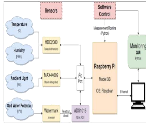
Figure 6: Sensor system block diagram [3]
