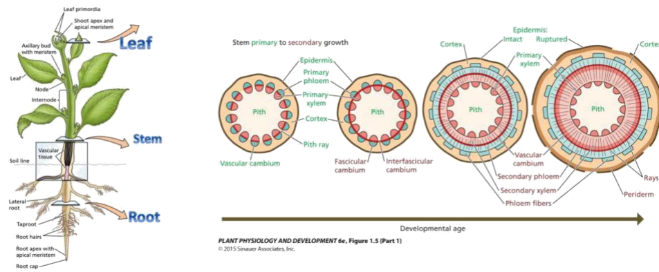
Figure 3: Plant stem structure
