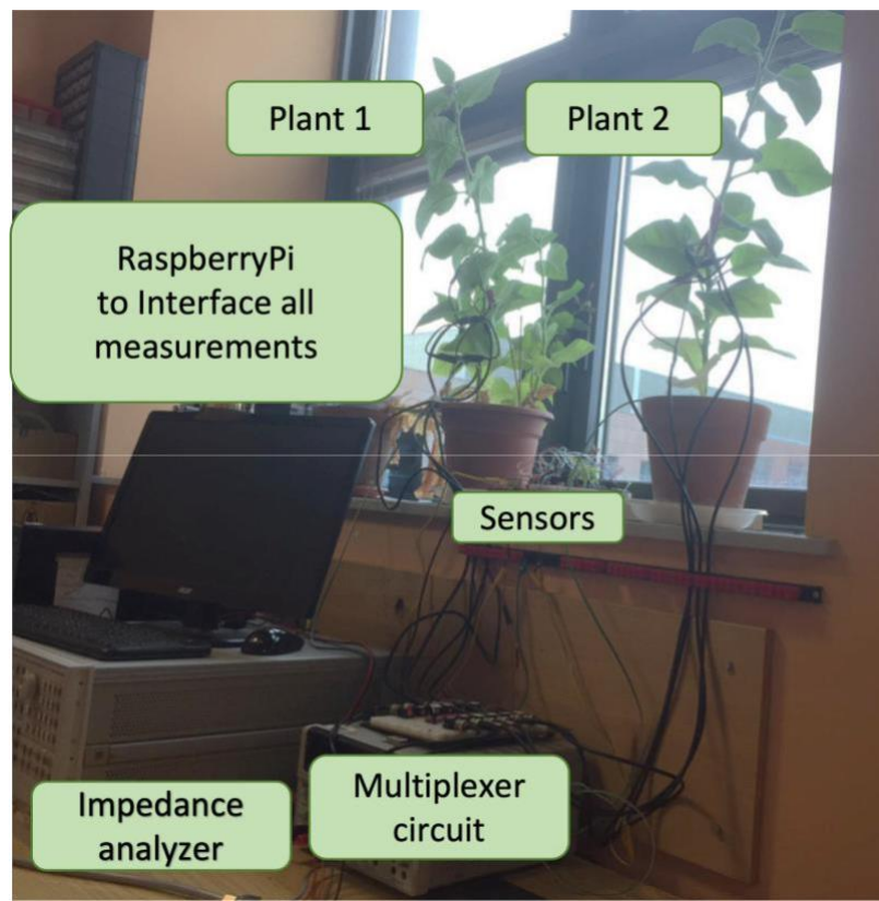
Figure 11: Continuous monitoring system depicting two plants monitored simultaneously in Turin, Italy.
