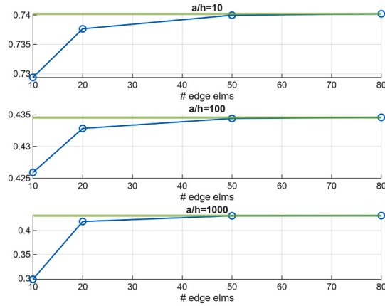
Fig. 4. ZZen-Q FE solution vs en-RZT exact solution convergence, L0 plate, non-dimensional maximum deflection \bar{w} .
