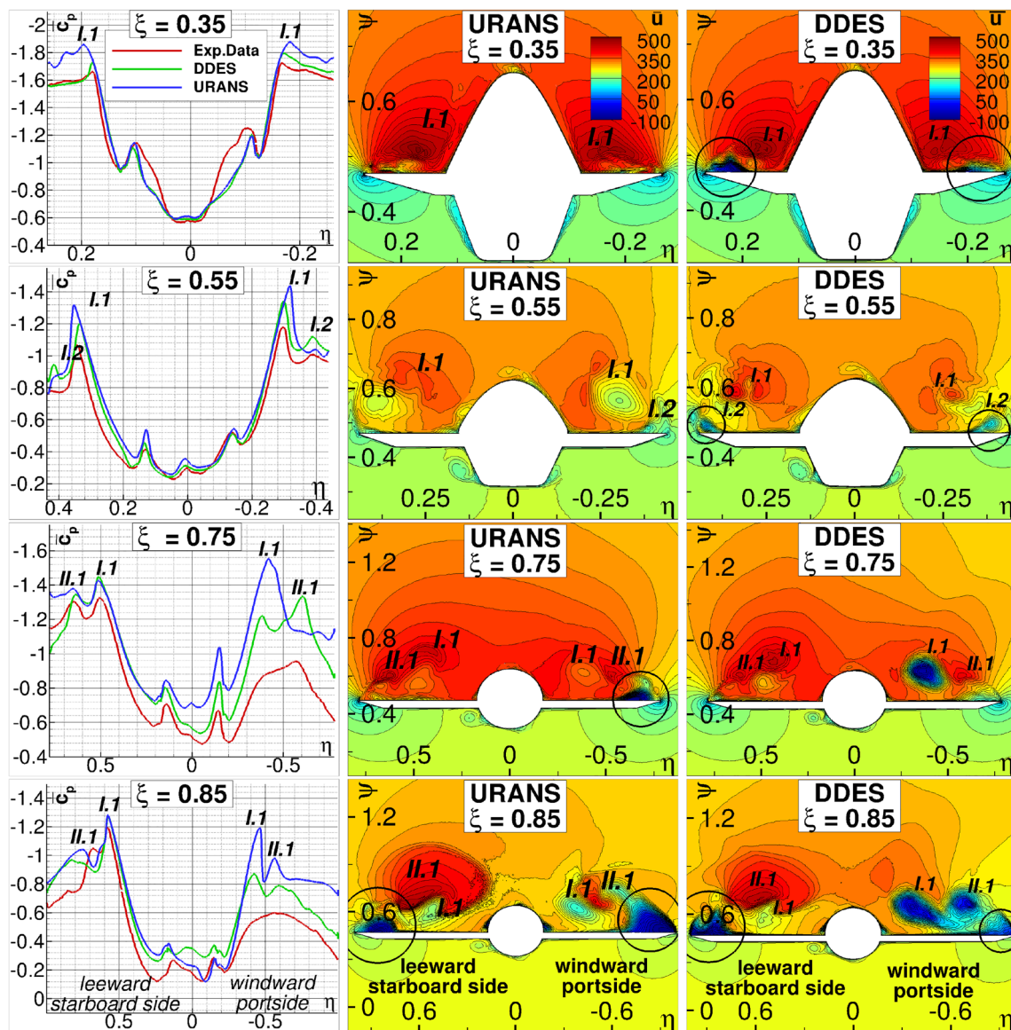
Fig. 8 Mean surface \overline{c_p} distribution and mean x-velocity \overline{u} [m/s] contour plots at chordwise locations \xi = 0.35, 0.55, 0.75, 0.85 , comparison between experimental data, URANS and DDES with \alpha = 20^\circ and \beta = 5^\circ
