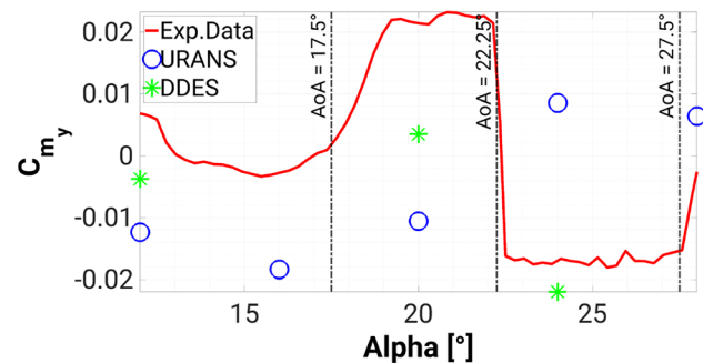
(c) Pitching moment coefficient over AoA
