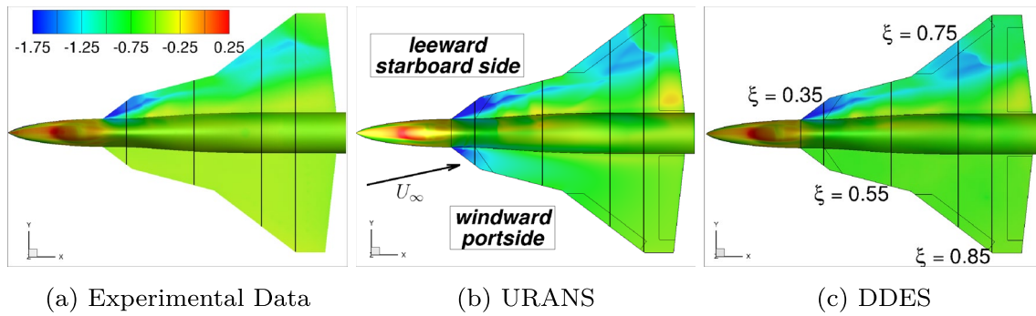
Fig. 10 Mean surface coefficient of pressure \overline{c_p} , comparison between experimental data, URANS and DDES results with \alpha = 24^\circ and \beta = 5^\circ
