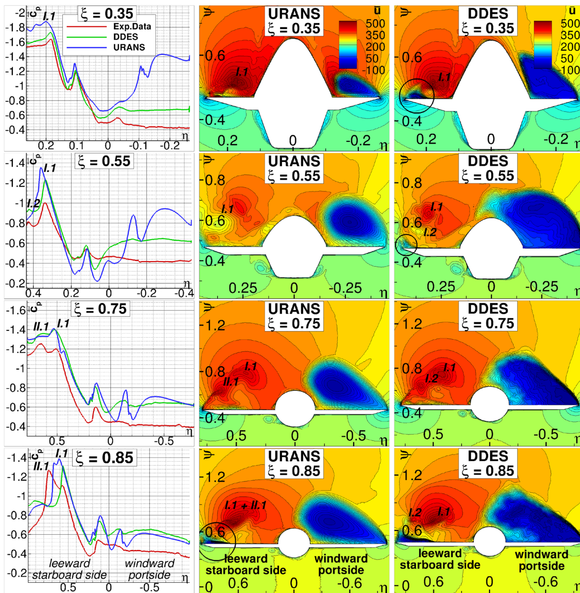
Fig. 11 Mean surface \overline{c_p} distribution and mean x-velocity \overline{u} [m/s] contour plots at chordwise locations \xi = 0.35, 0.55, 0.75, 0.85 , comparison between experimental data, URANS and DDES with \alpha = 24^\circ and \beta = 5^\circ
