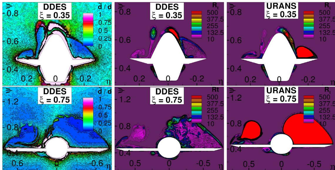
Fig. 12 Instantaneous hybrid length scale over RANS length scale (left) and instantaneous turbulent eddy viscosity, represented by R_t at chordwise locations \xi = 0.35, 0.75 , comparison between URANS and DDES with \alpha = 24^\circ and \beta = 5^\circ
