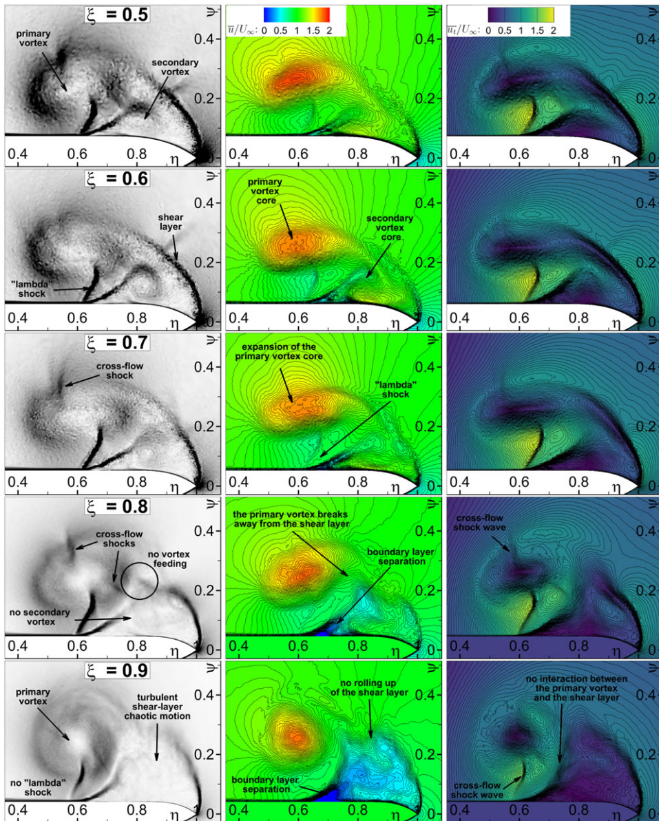
Figure 9. Mean density gradient magnitude ||\nabla\rho|| , mean normalised x -direction velocity \bar{u}/U_\infty and mean normalised in-plane tangential velocity \bar{u}_t/U_\infty distribution, IDDES results at chordwise locations \xi = 0.5, 0.6, 0.7, 0.8, 0.9 [12].
