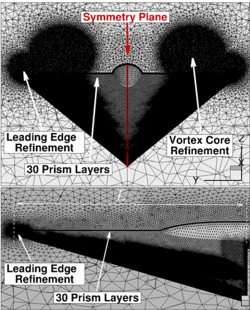
Figure 1. VFE-2 geometry and mesh.
