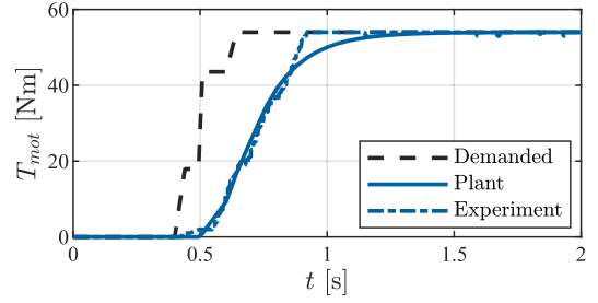
FIGURE 3. Time profiles of the reference motor torque ('Demanded'), torque from the high-fidelity simulation model ('Plant'), and experimentally measured torque ('Experiment', from the inverter current) along a tip-in test.
