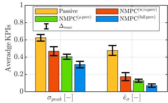
FIGURE 15. \sigma_{peak} and \hat{e}_\sigma for the rear left corner, across the 24 experimental speed bump tests covering the considered NMPC configurations, where the histograms refer to the average values and the error bars to the range of the respective KPI.
