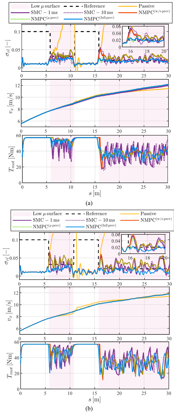
FIGURE 9. Performance comparison of the considered SMCs and NMPCs in terms of \sigma_H , v_x , and T_{\text{mot}} profiles, along sections of (a) an ISO class B road and (b) an ISO class C road, with varying friction levels.
