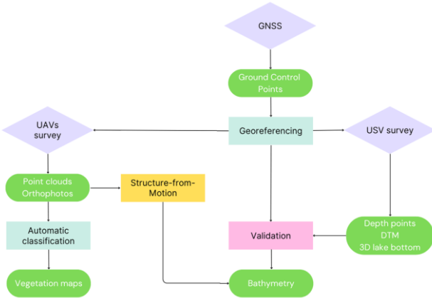
Figure 4. Methodological workflow.
