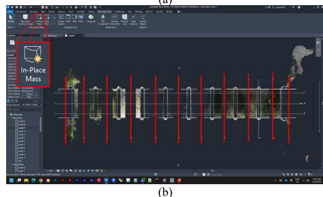
Figure 6. Mass modelling of deck profile (a). Longitudinal and Cross section lines on point cloud (b).
